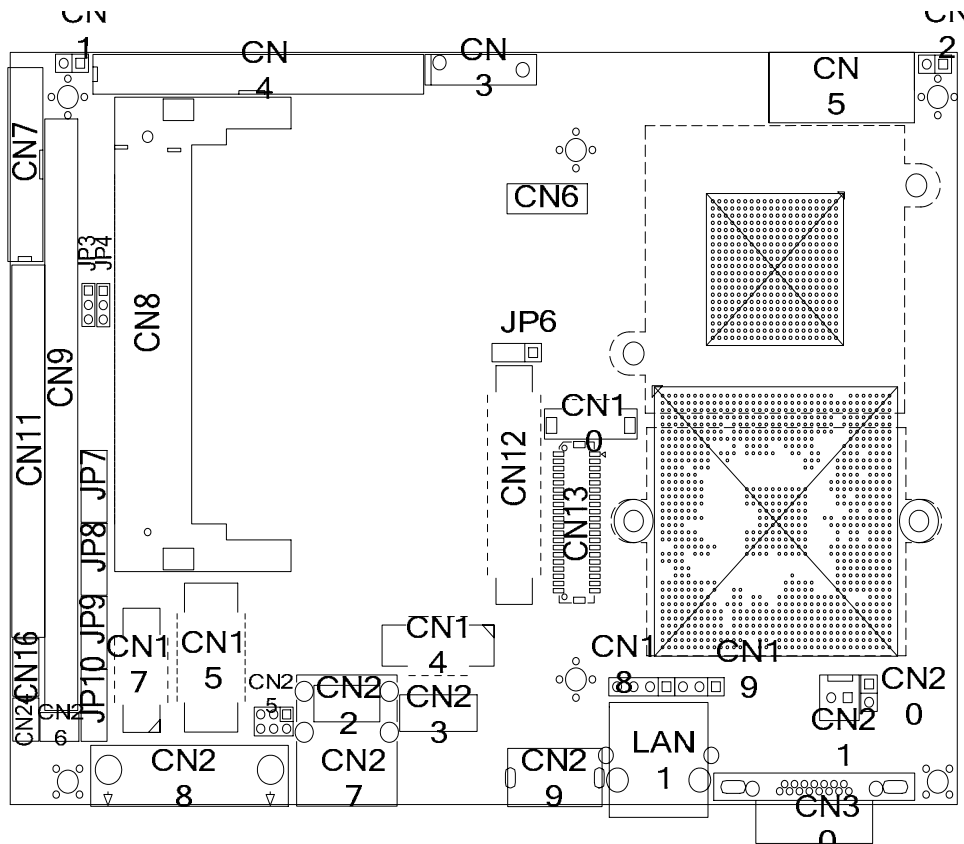
Component Side
