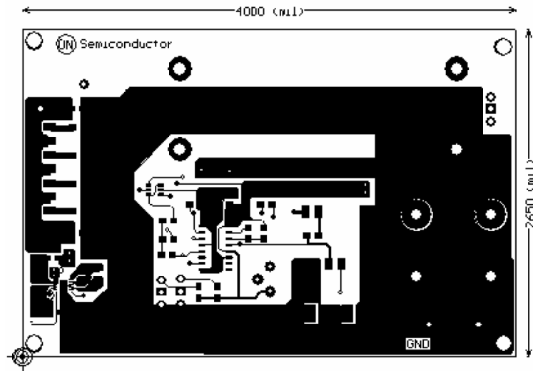
Figure 4. Top Layer
