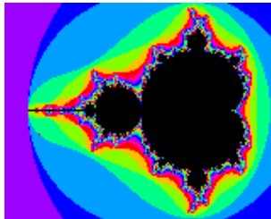
Figure 11.35.: Mandelbrot
