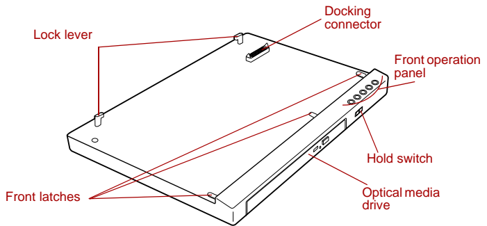
Figure 8-11 Front and left side the libretto DVD Dock
