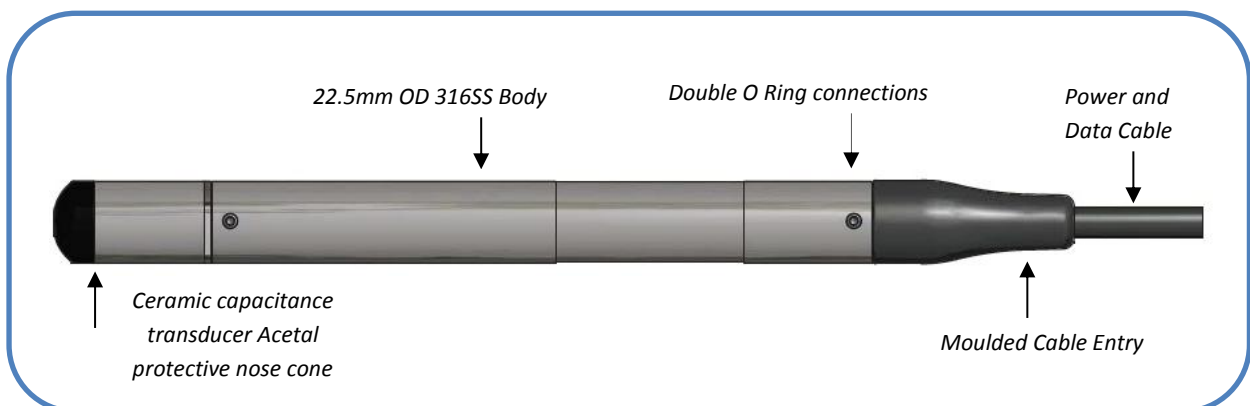
PS7000 Primary Elements
