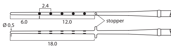
Figure 22 Insertion Test Device
