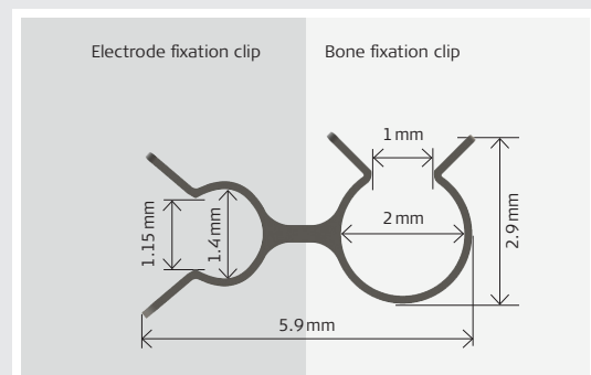
Figure 54 Dimensions of the Fixation Clip
