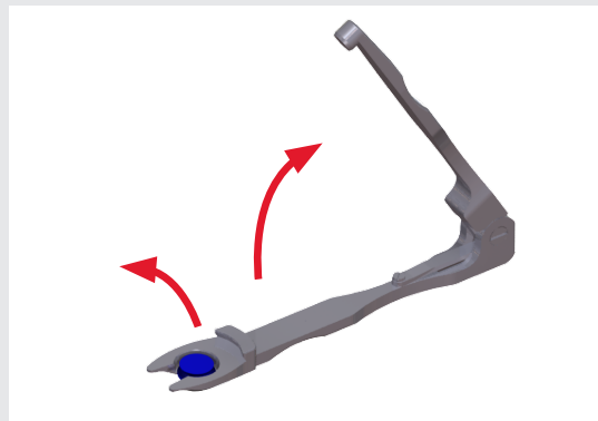
Figure 70 Opening the instrument and removing the magnet from the instrument tip
