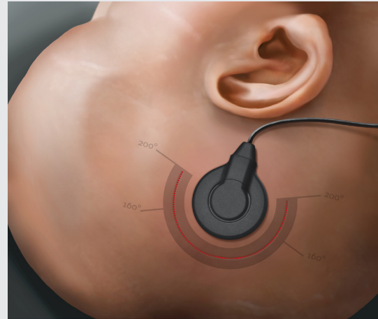
Figure 66 Showing recommended incision line with MAX Coil S in non-sterile environment
