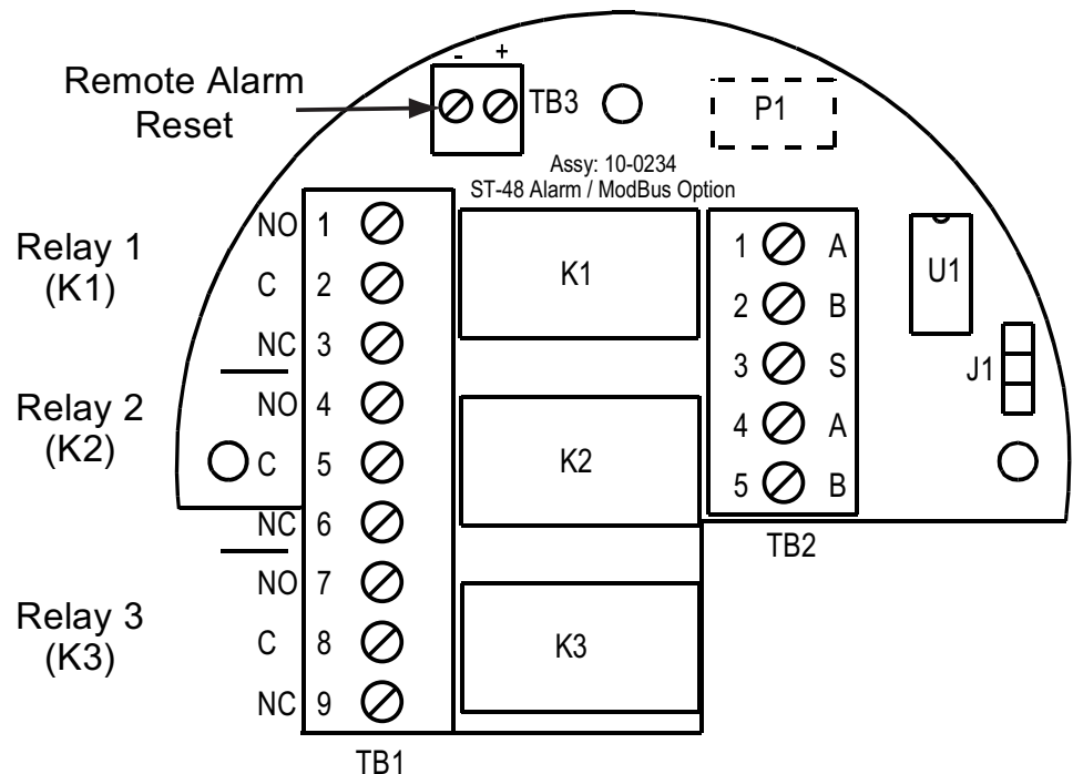
Figure 15 Relays/Remote Alarm Reset Connections - Relays/MODBUS Option PCB
