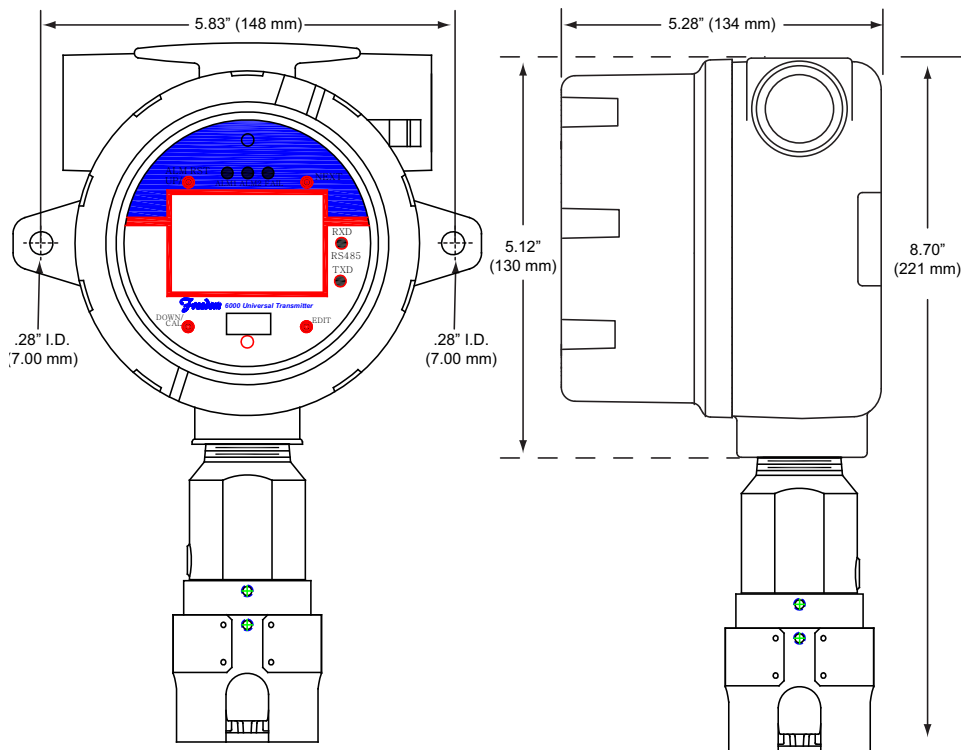
Figure 6 Device Mounting Dimensions - Aluminum
