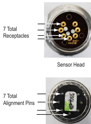
Figure 27 Combustible (LEL) Sensor Assembly Alignment - 6.0V Cat-bead
