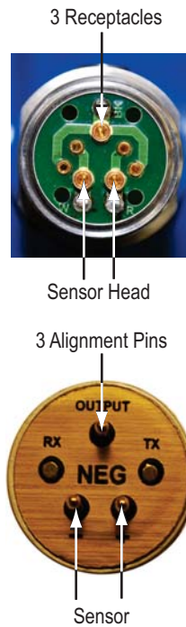
Figure 25 Combustible (LEL) Sensor Assembly Alignment - 4.25V IR
