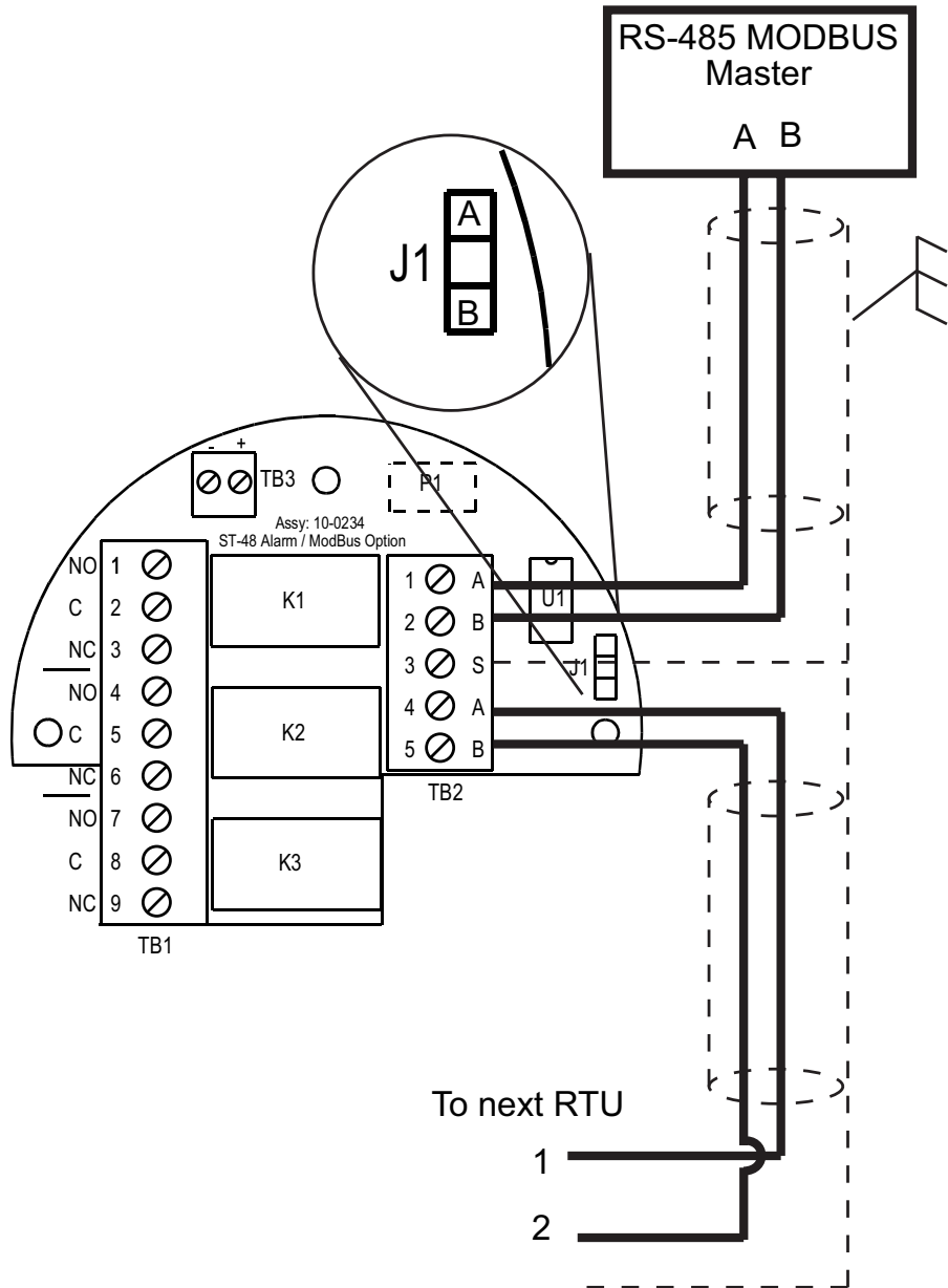
Figure 16 MODBUS Connections - Relays/MODBUS RS-485 Option PCB
