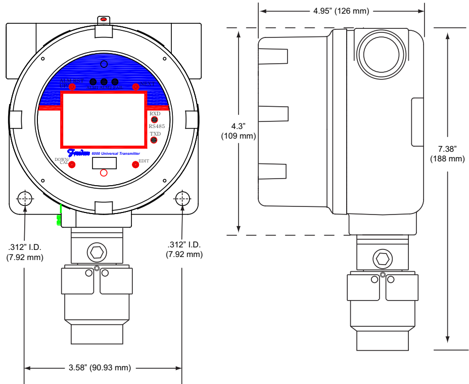
Figure 7 Device Mounting Dimensions Stainless Steel
