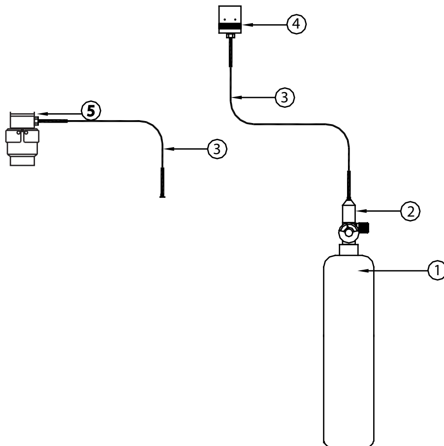
Figure 52 Combustible (LEL) Calibration Hookup Methods
