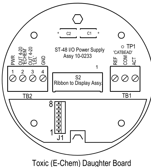
Figure 19 Toxic (E-Chem) Sensor Head Connection – ClassI, Division2
