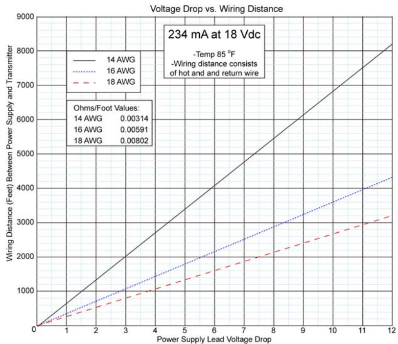
Figure 3 Wiring Distance Reference Chart @ 18VDC
