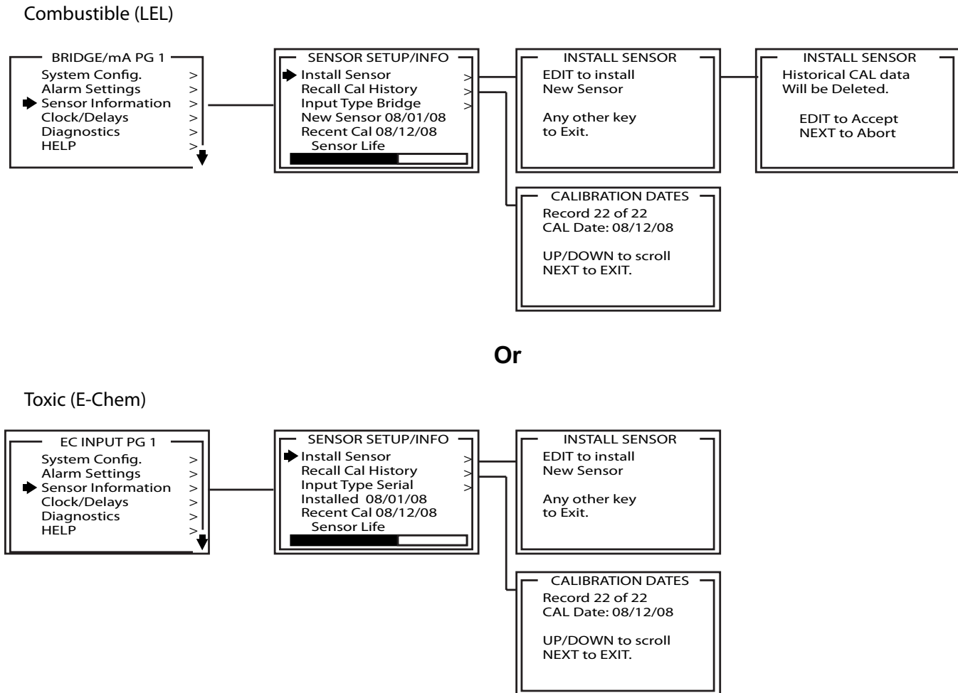
Figure 32 Configuration Menu - Sensor Info. Combustible (LEL) & Toxic (E-Chem)
