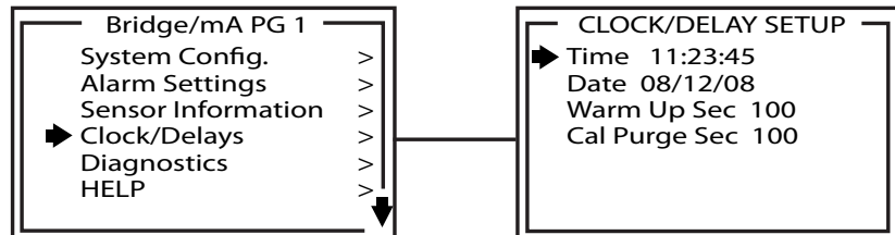
Figure 33 Configuration Menu - Clock/Delays Setup
