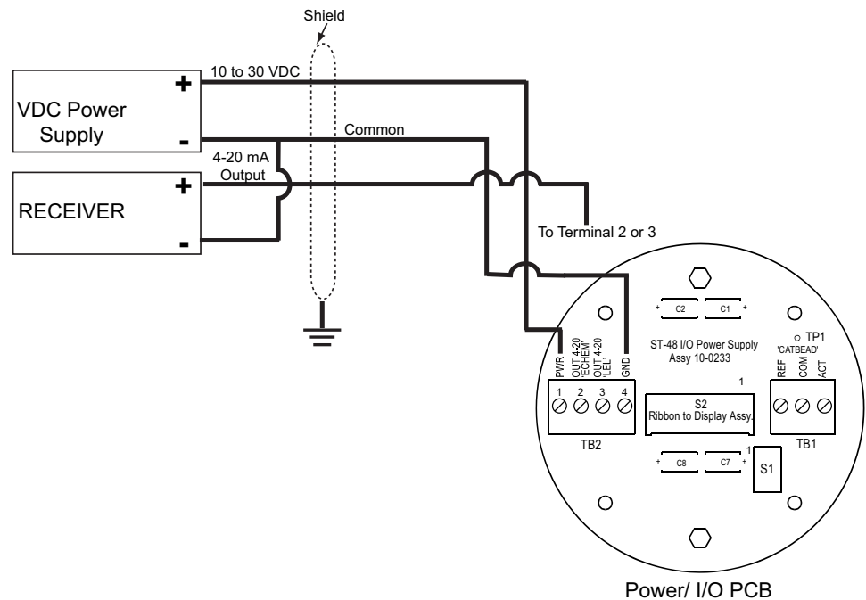
Figure 14 Connection for 3-Wire
