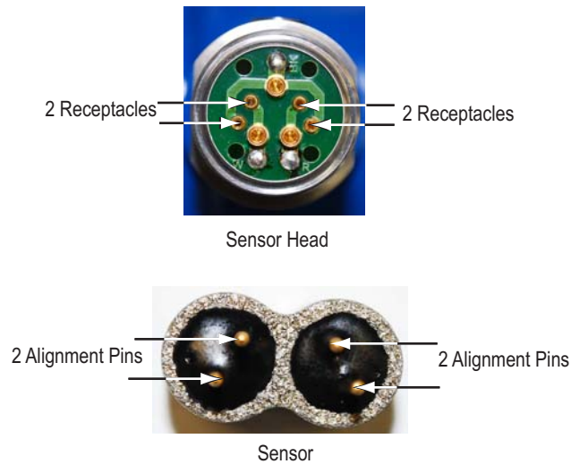
Figure 26 Combustible (LEL) Sensor Assembly Alignment - 5.5V Cat-bead
