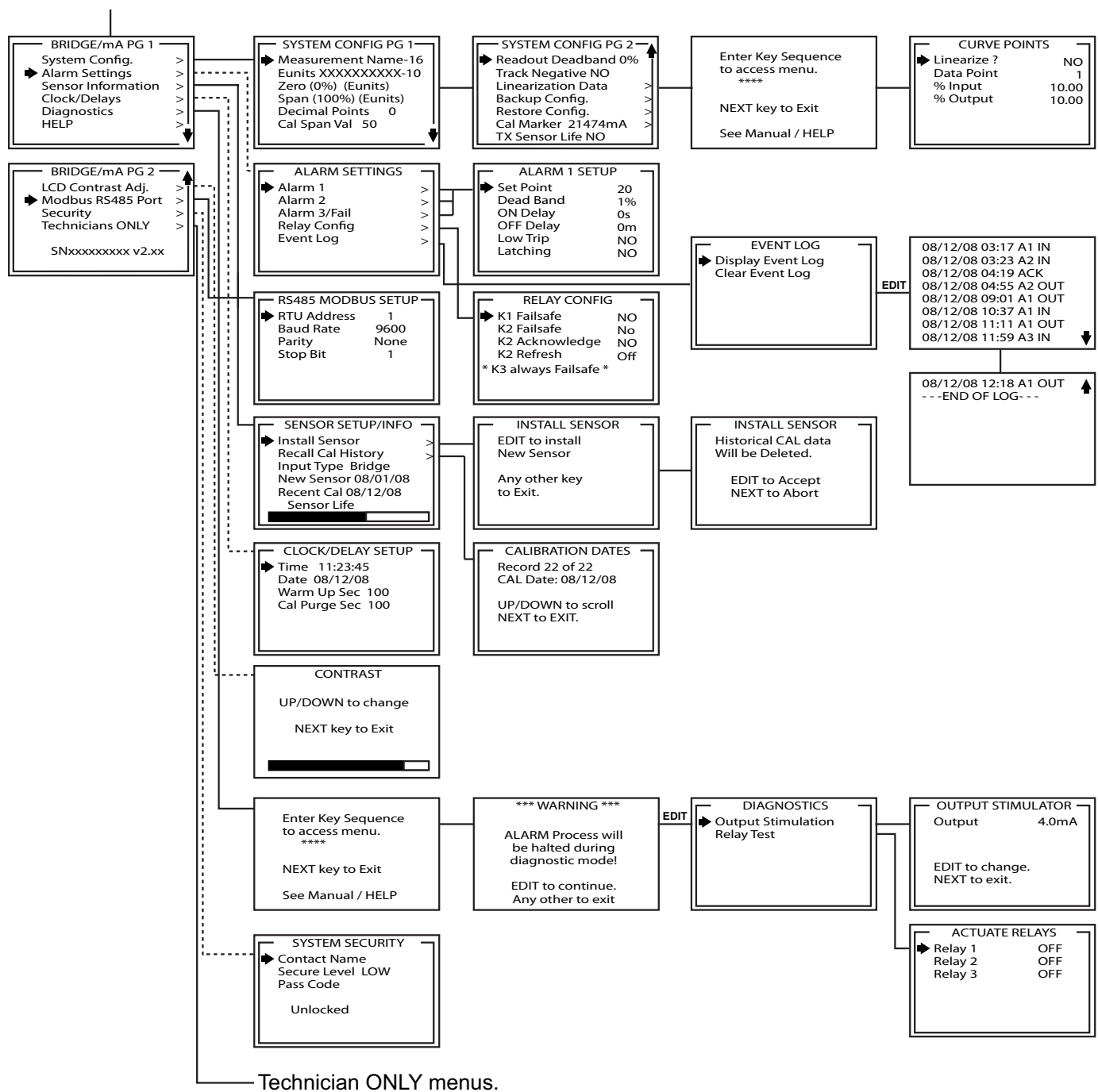
Figure 28 Configuration Menu Structure - Combustible (LEL) Sensor Head
