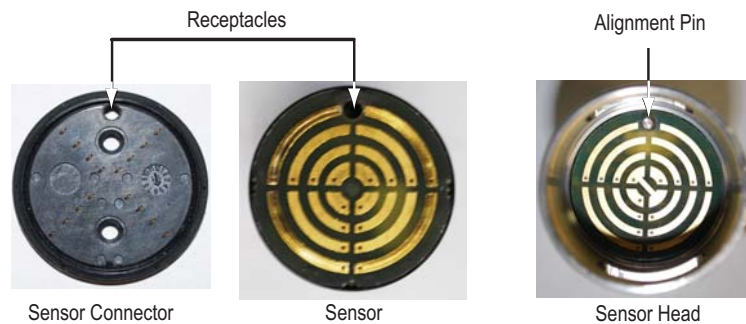
Figure 21 Toxic (E-Chem) Sensor Assembly Alignment
