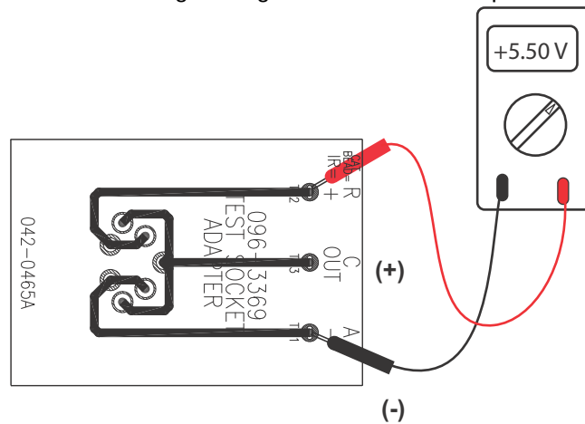
Figure 10 Measure the Voltage Using the Test Socket Adapter
