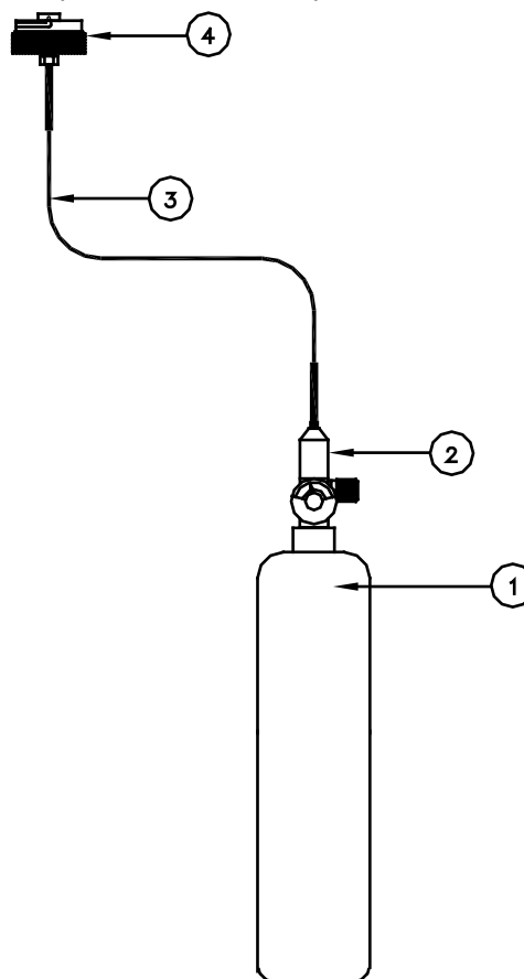
Figure 53 Toxic (E-Chem) Calibration Hookup Method
