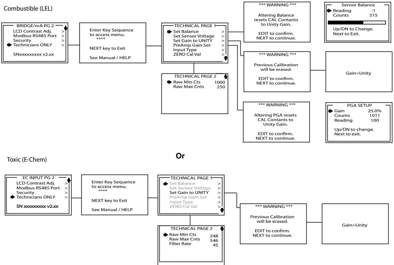
Figure 41 Configuration Menu - Technicians Only
