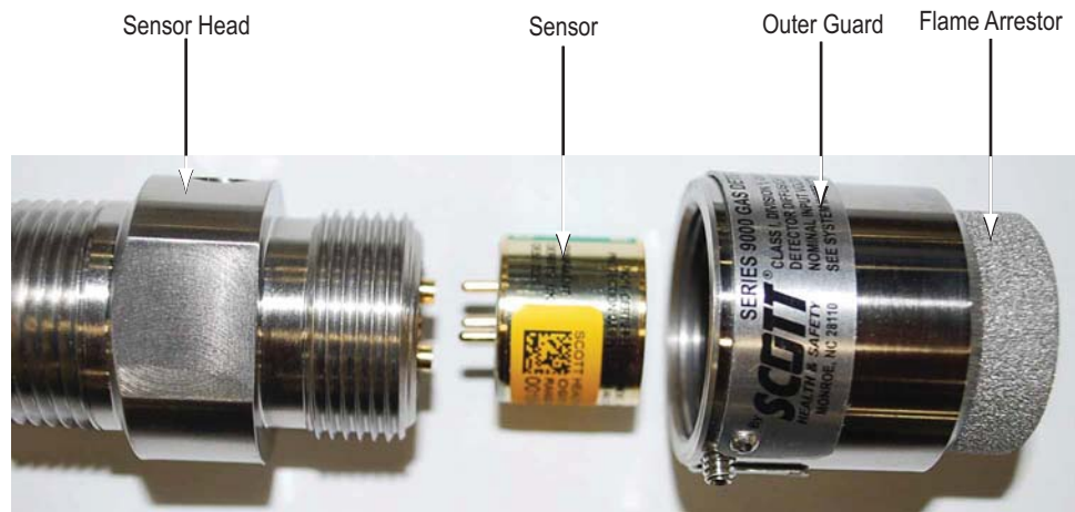
Figure 22 Combustible (LEL) Sensor Assembly – 4.25V
