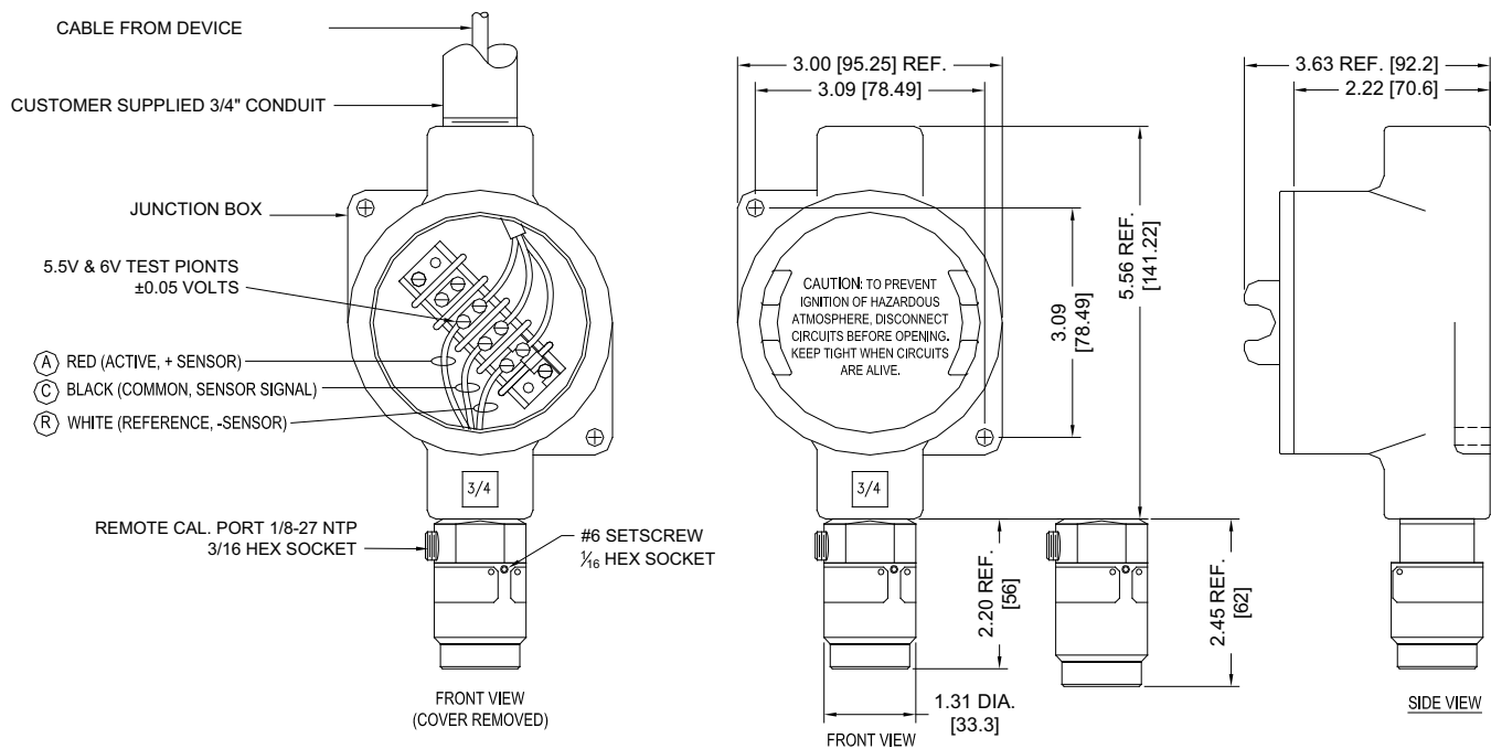
Figure 8 Remote Sensor Junction Wiring and Mounting - Combustible
