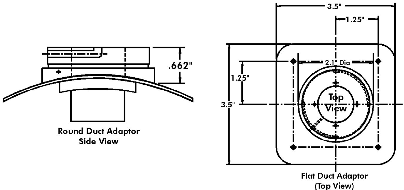
Figure 13 Duct Mount Adapter Mounting - Toxic (E-Chem) Sensor Head
