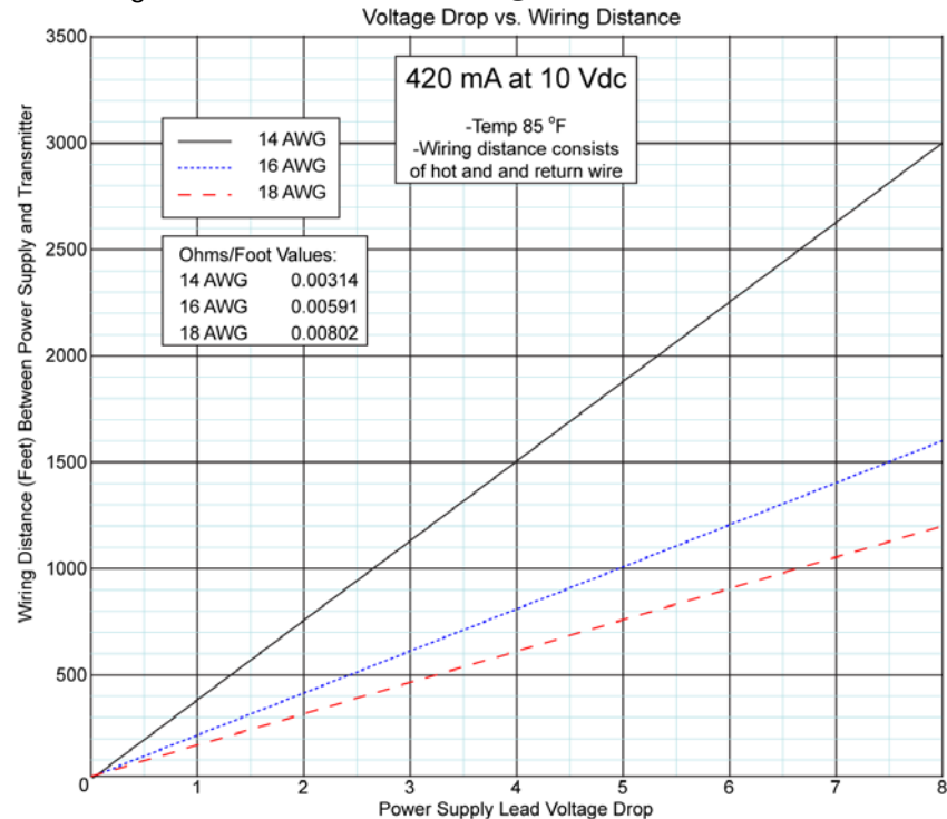
Figure 4 Wiring Distance Reference Chart @ 10VDC
