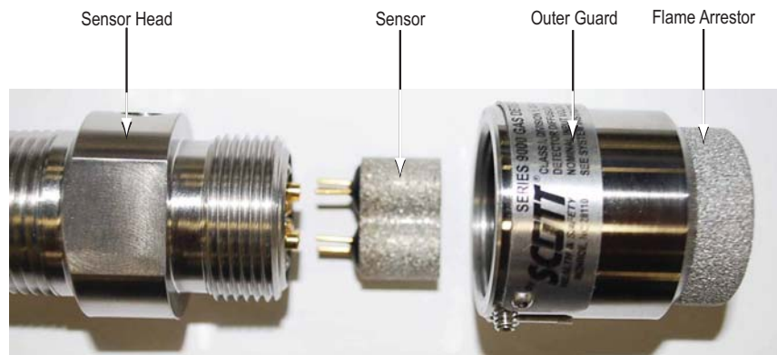
Figure 23 Combustible (LEL) Sensor Assembly – 5.5V
