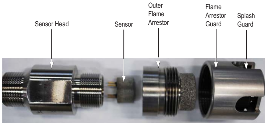
Figure 24 Combustible (LEL) Sensor Assembly – ATEX Approved
