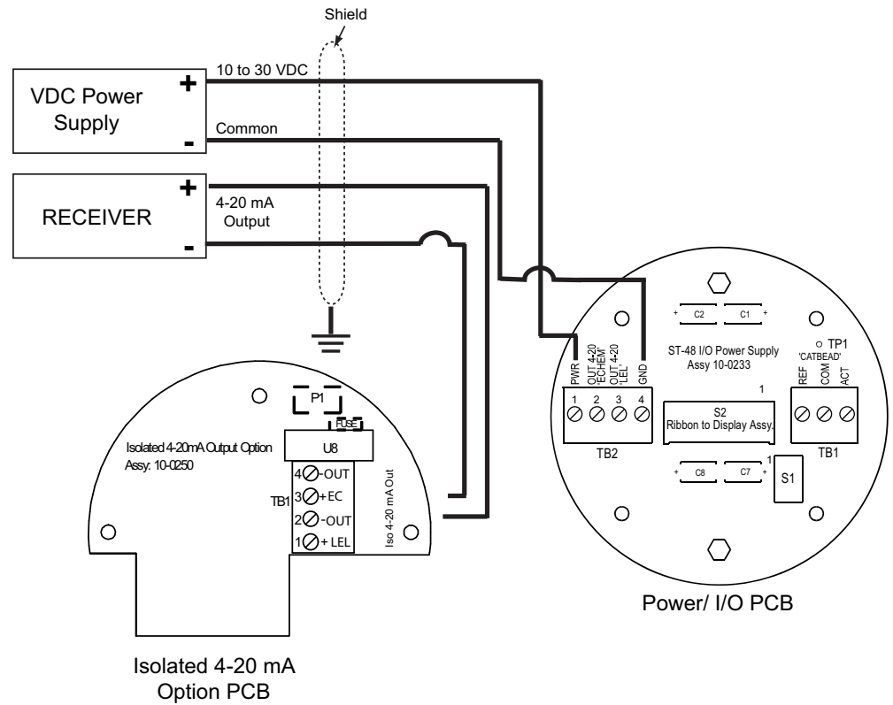
Figure 17 4-20mA Connections - Isolated 4-20mA Option PCB
