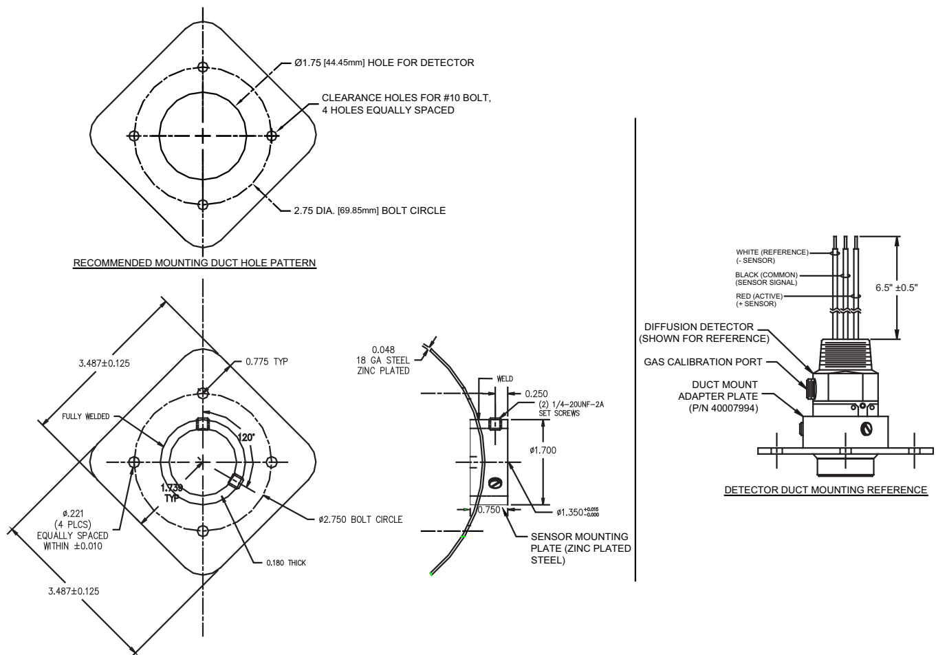
Figure 12 Duct Mount Adapter Mounting - Combustible (LEL) Sensor Head
