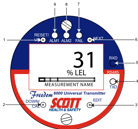
Figure 49 Text and Numerical Display
