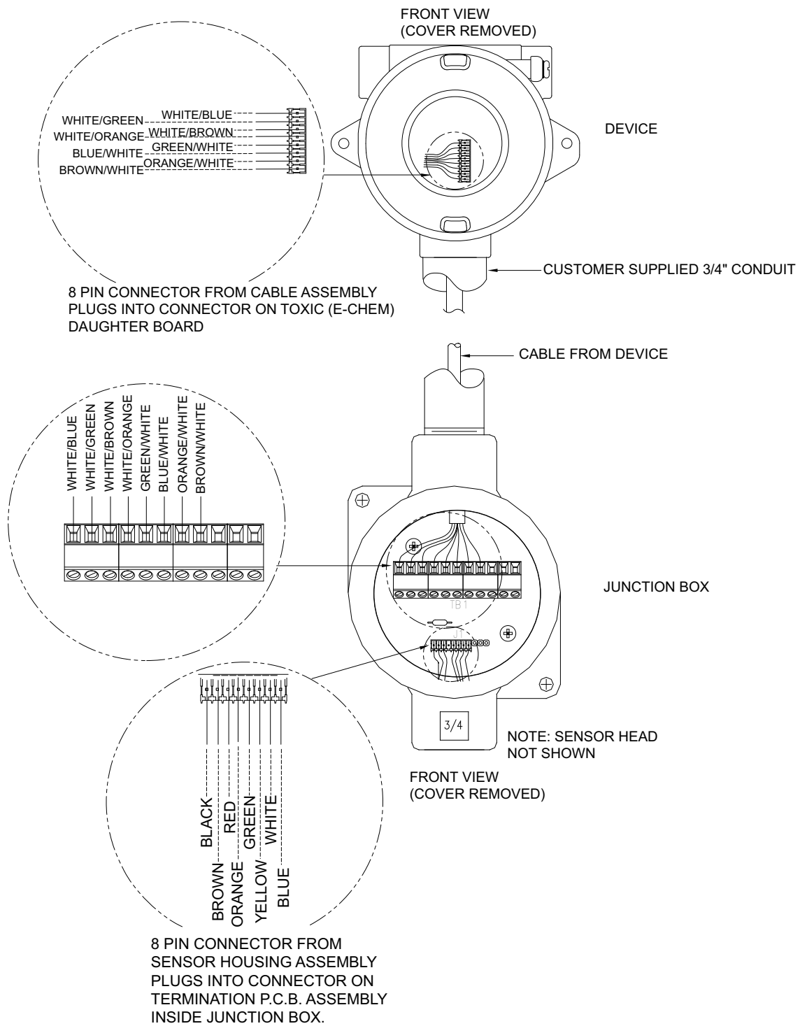
Figure 11 Remote Sensor Junction Wiring - Toxic
