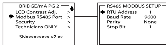
Figure 37 Configuration Menu - MODBUS RS-485 Port
