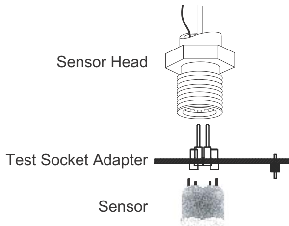
Figure 9 Using a Test Socket Adapter
