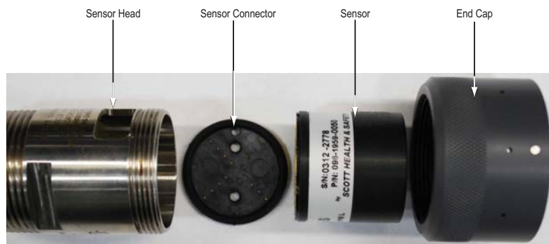
Figure 20 Toxic (E-Chem) Sensor Head Assembly – ClassI, Division2
