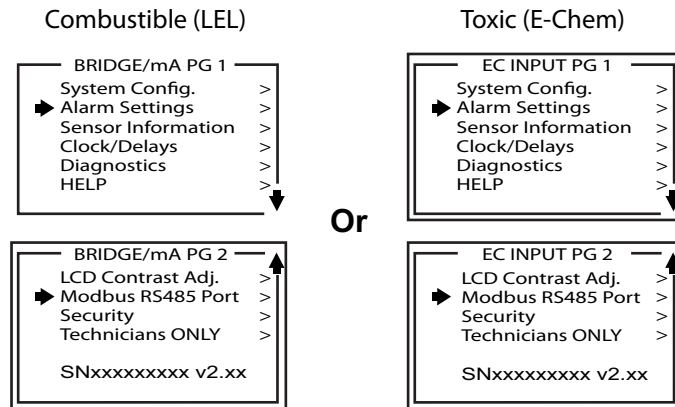
Figure 29 Configuration Menu - Setup Display Combustible (LEL) & Toxic (E-Chem)
