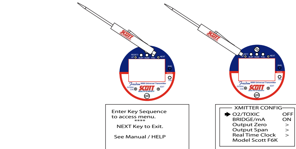
Figure 39 Configuration Menu - Transmitter Configuration
