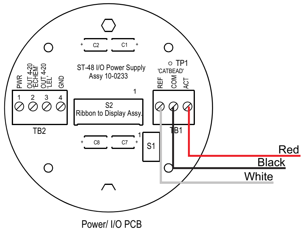
Figure 18 Combustible (LEL) Cat-bead and IR Sensor Head Connections
