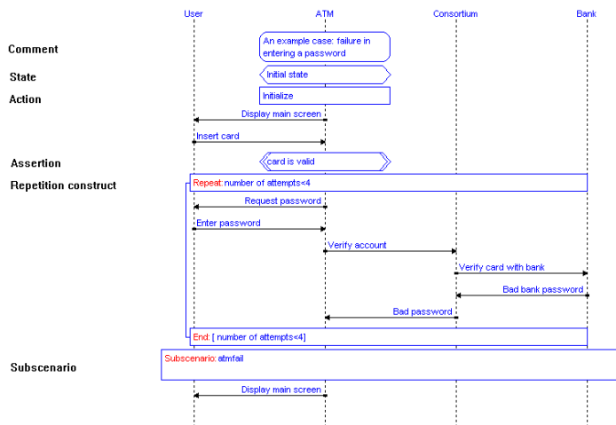
Fig. 2. Elements of SCED scenario notation
