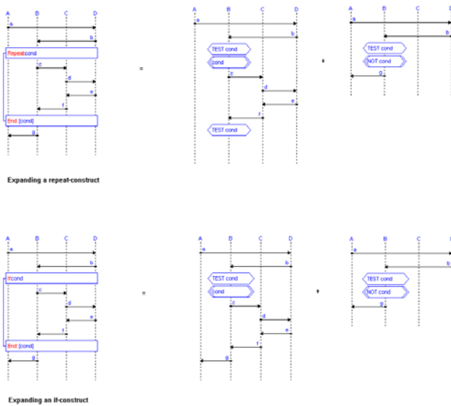
Fig. 3. Dissolving if- and repeat-constructs into simple scenarios.
