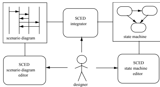
Fig. 1. General structure of SCED
