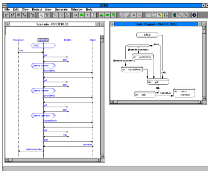
Fig. 5. Synthesizing operation descriptions from scenarios.
