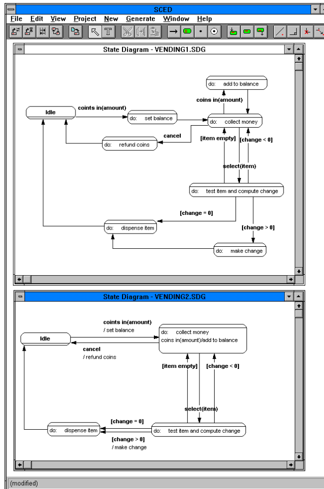
Fig. 8. Transforming a state machine into OMT notation.
