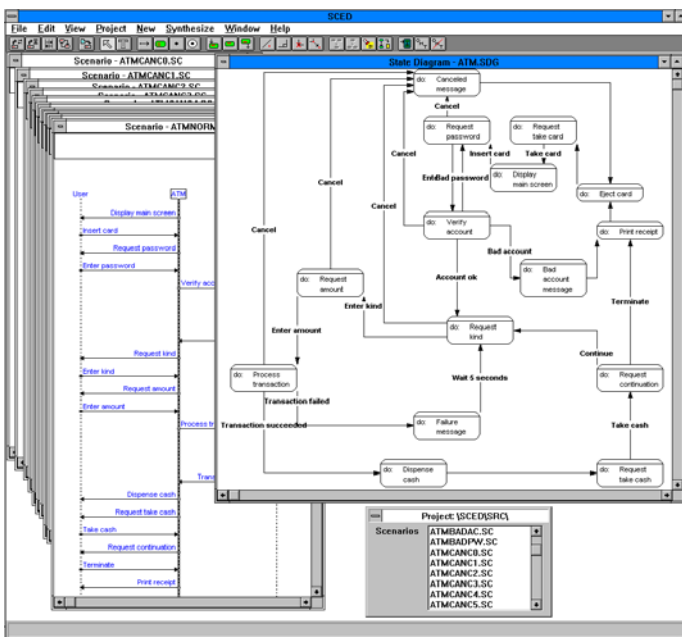
Fig. 4. Scenario diagrams and a synthesized state machine in SCED
