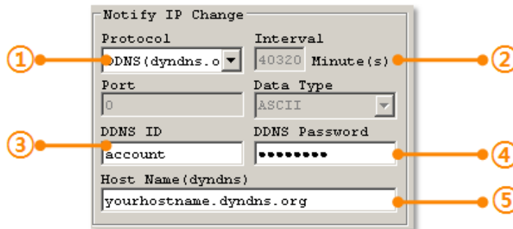
Figure 7-1 setting DDNS
