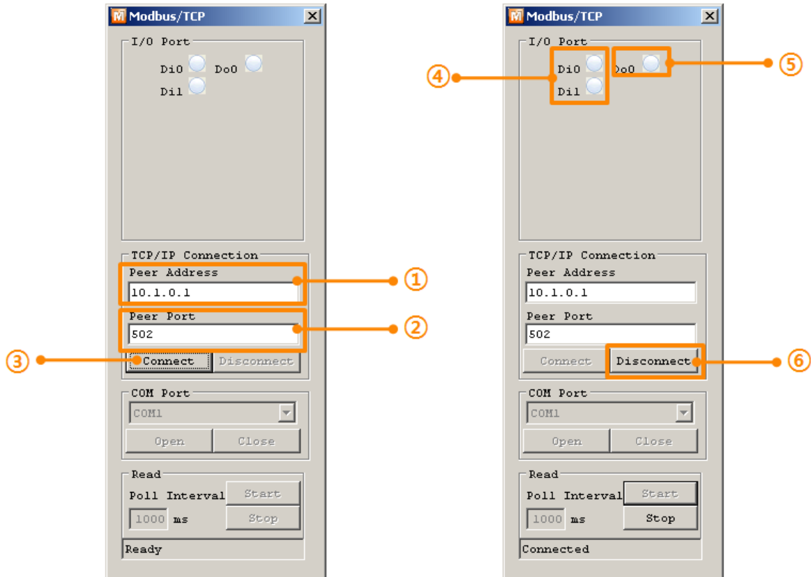
Figure 2-4 Modbus/TCP test
