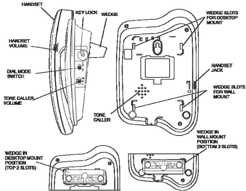
Figure 2: Phone Base
