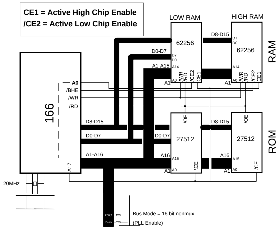
166: 16 Bit Non-Multiplexed Bus With Byte Memories
