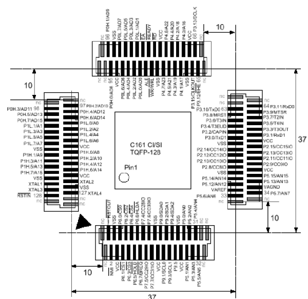
QuadConnect Footprint For 128TQFP Packages
