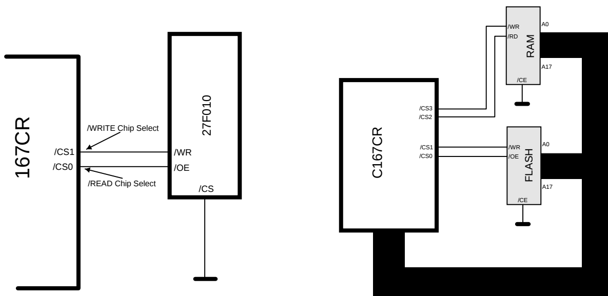
READ & WRITE Chip Selects
