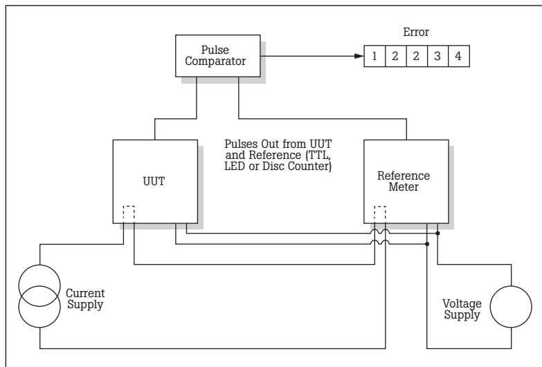
Figure 1. A typical energy meter calibration setup.
