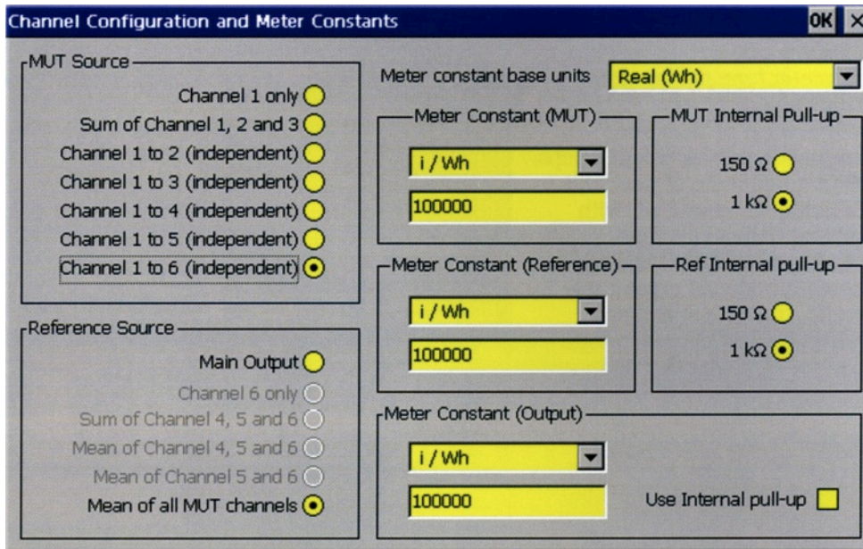
Figure 12. Channel Configuration and Meter Constants screen.
