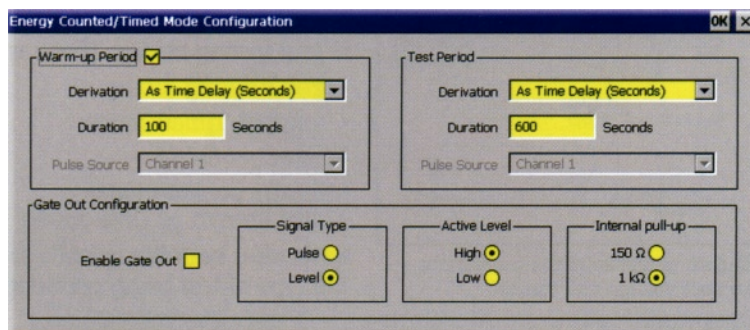
Figure 9. Energy Counter/Timer mode configuration screen.
