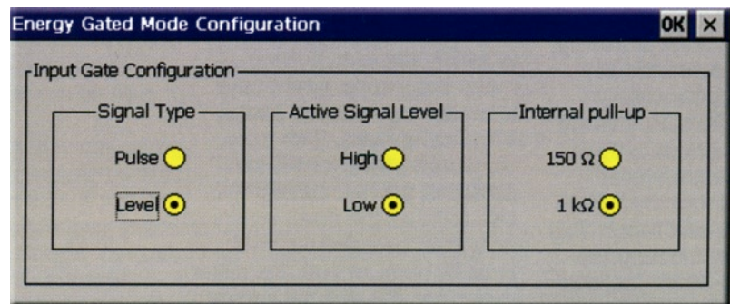
Figure 10. Energy Gated mode configuration screen.
