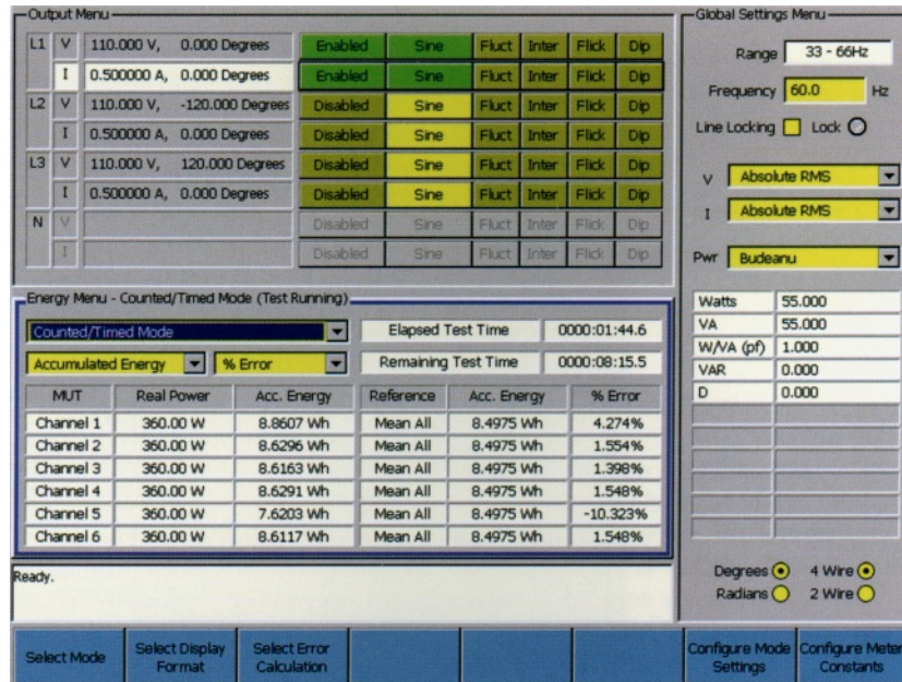
Figure 13. The 6100's Output Status screen.
