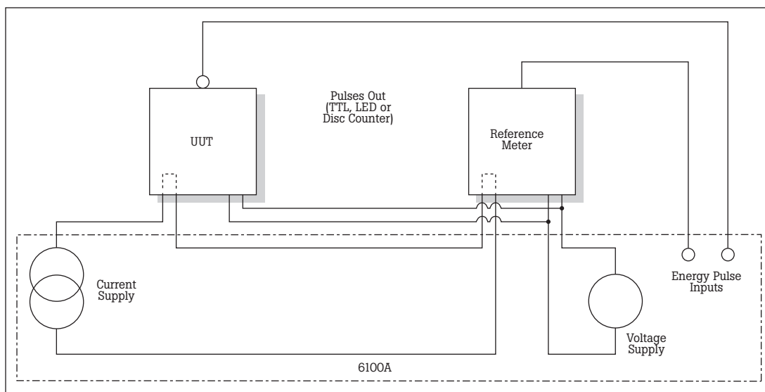
Figure 3. The 6100A Electrical Power Standard eliminates the need for comparators in the calibration setup.
