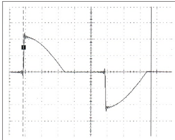
Figure 6. Phase fired signal.
