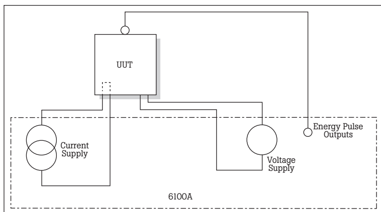
Figure 4. Using a 6100A Electrical Power Standard to eliminate the comparator and reference meter, as well as a supply for both voltage and current.
