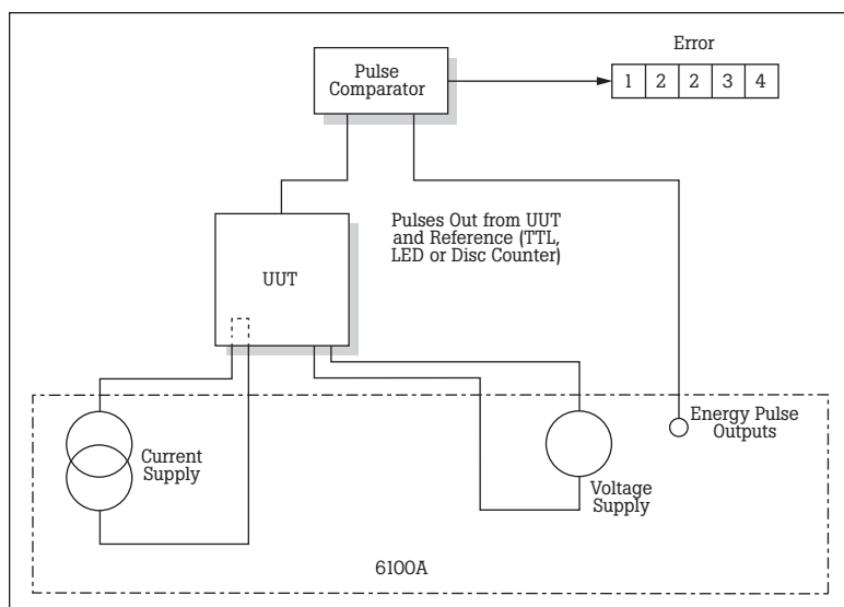
Figure 2. An energy meter calibration setup using a 6100A Electrical Power Standard.
