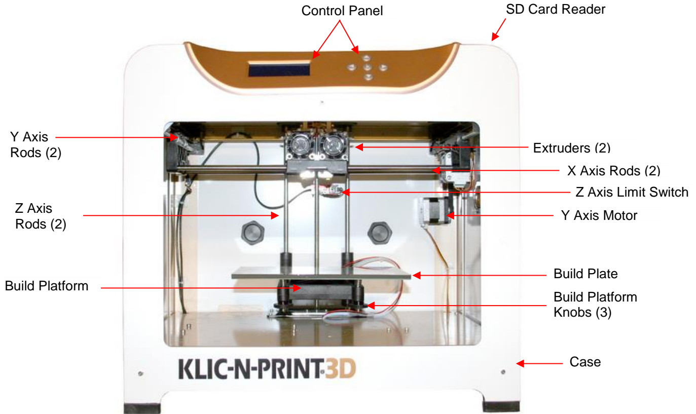
Front of KNP3D
