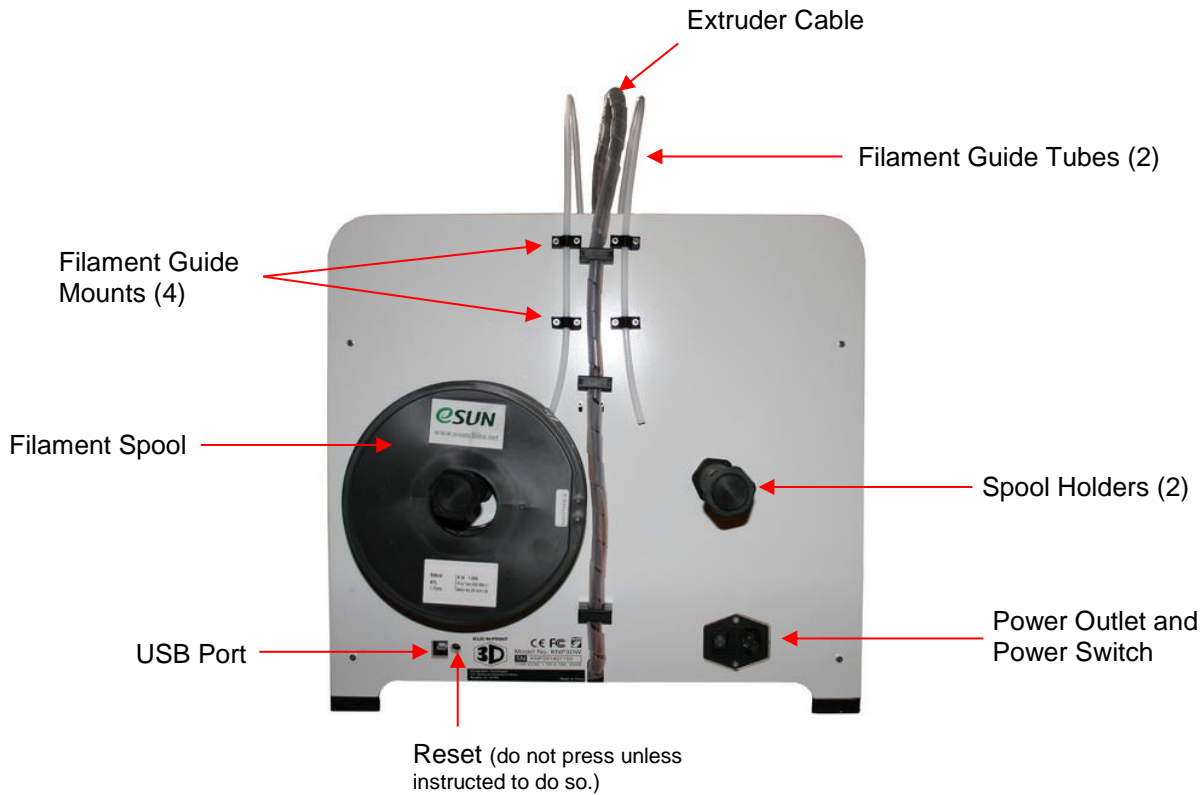
Back of KNP3D
