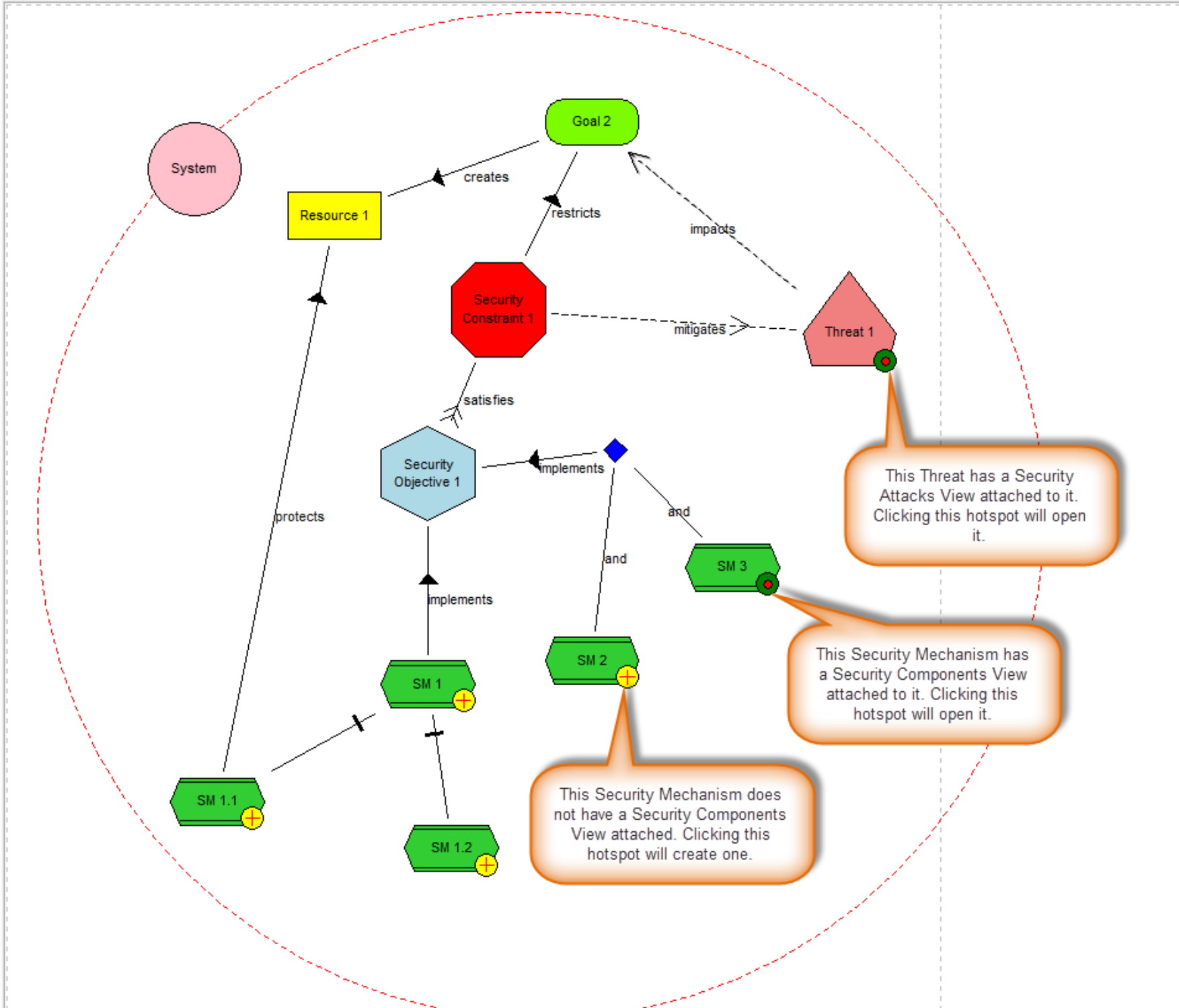
Figure 20. Demonstration of the Security Requirements View and Security Mechanisms'/Threats' hotspots.
