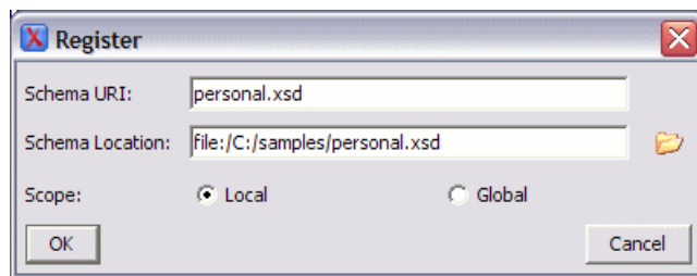
Figure 10.4. Register Dialog
