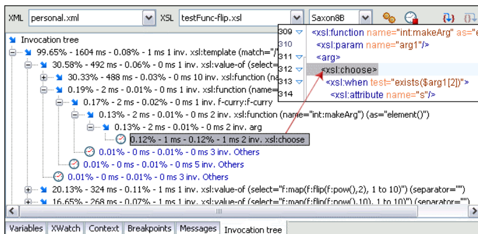
Figure 8.3. Source backmapping
