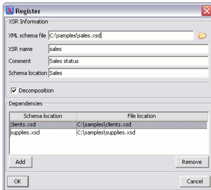
Figure 10.5. Register Dialog
