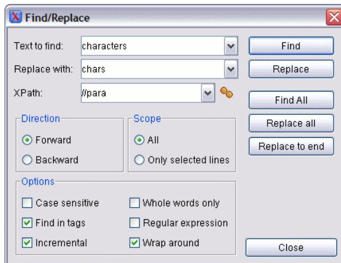
Figure 4.99. Find/Replace Dialog
