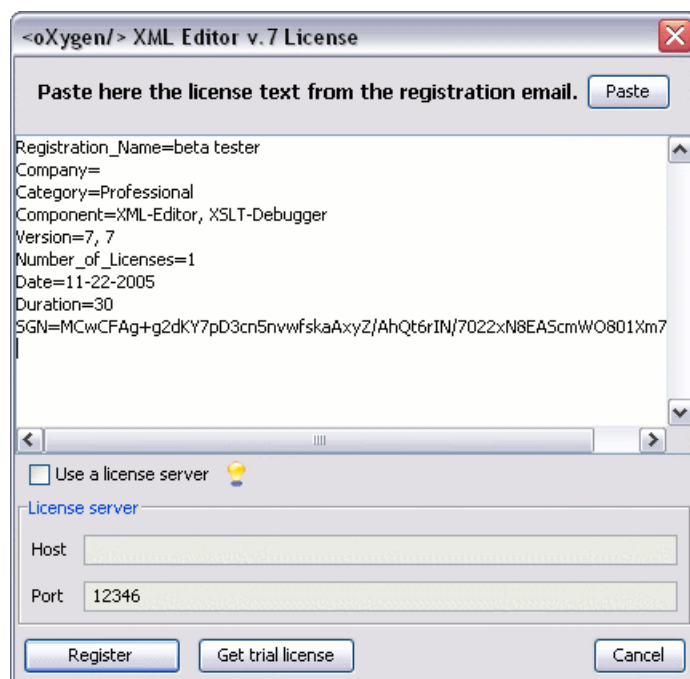
Figure 2.1. Registration Dialog
