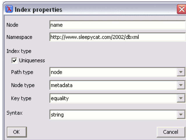
Figure 10.21. Adding/editing indices
