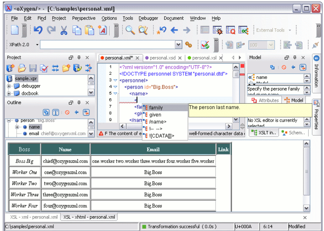
Figure 3.3. Editor perspective
