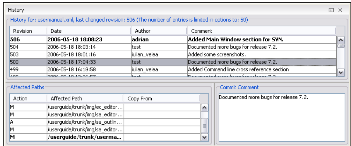
Figure 14.22. History view
