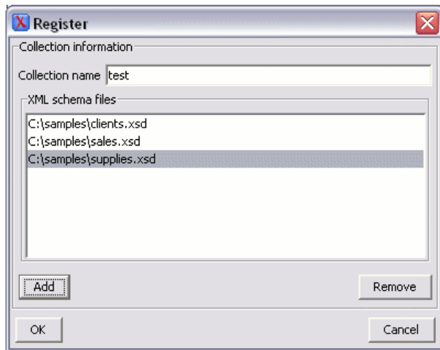
Figure 10.6. Register Dialog
