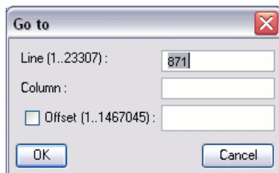
Figure 4.38. Go to
