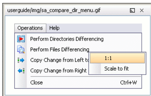
Figure 14.36. Image preview
