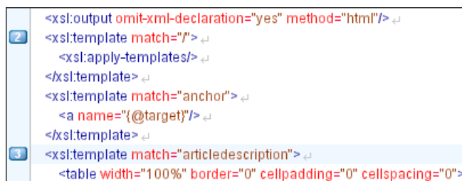
Figure 4.33. Editor Bookmarks
