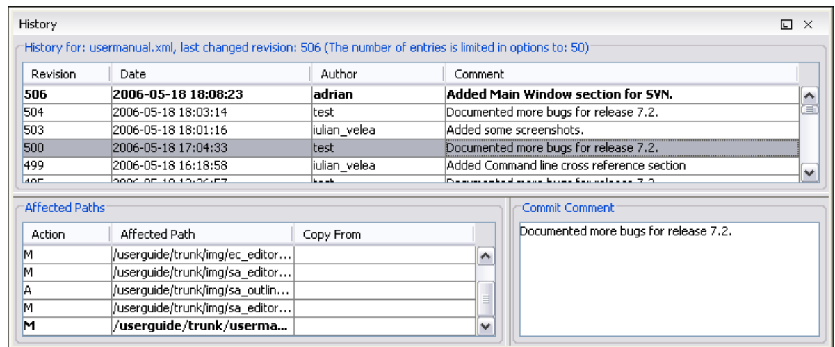
Figure 14.37. History view
