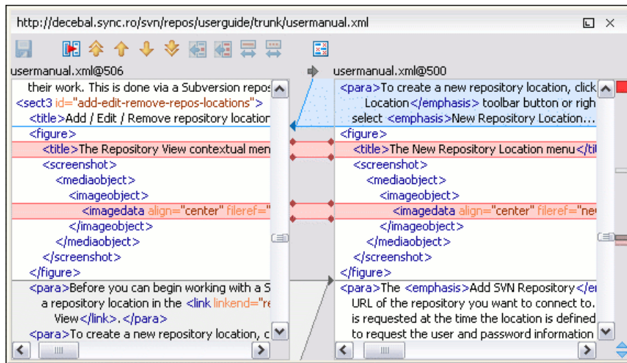
Figure 14.16. Compare View
