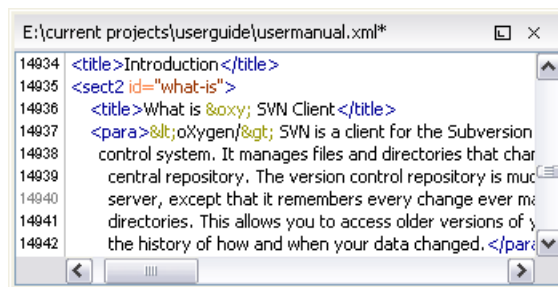
Figure 14.10. Editor view
