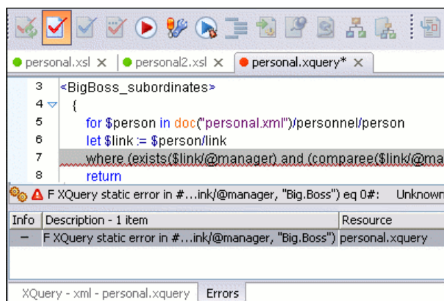
Figure 6.7. XQuery Validation
