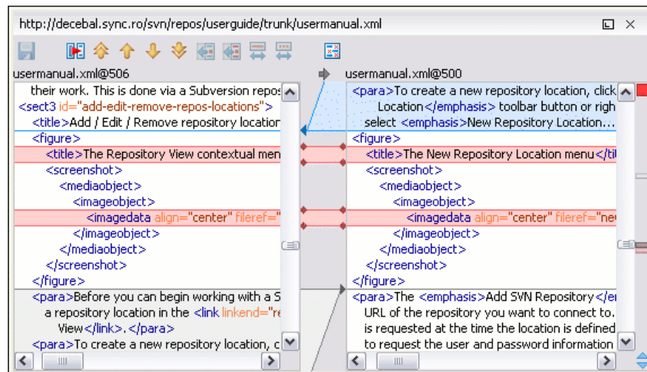
Figure 14.32. Compare view
