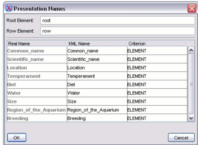
Figure 11.8. Presentation Names
