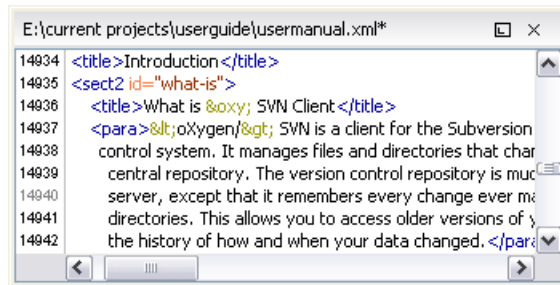
Figure 14.34. Editor view
