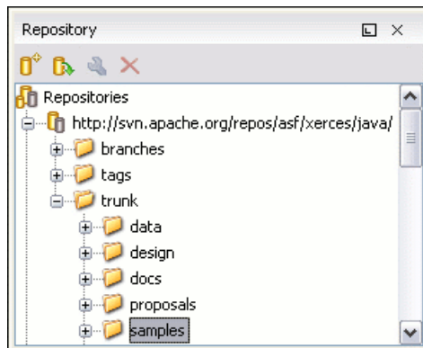
Figure 14.2. Repository View
