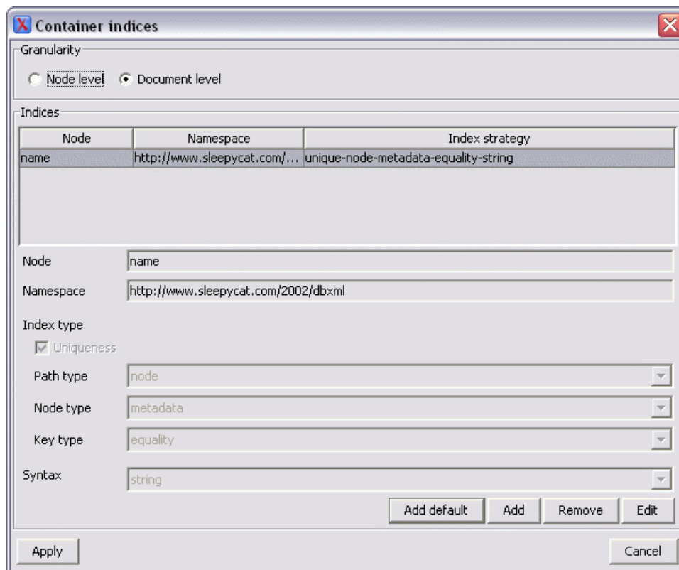
Figure 10.20. Container indices
