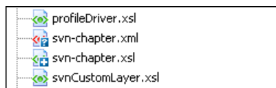
Figure 14.11. Unversioned / Added
