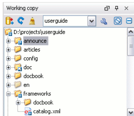
Figure 14.30.
