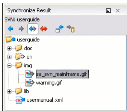
Figure 14.31. Synchronize view
