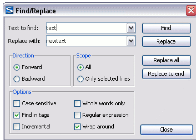
Figure 14.35. Find/Replace Dialog
