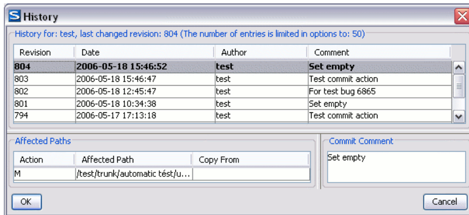
Figure 14.8. History dialog
