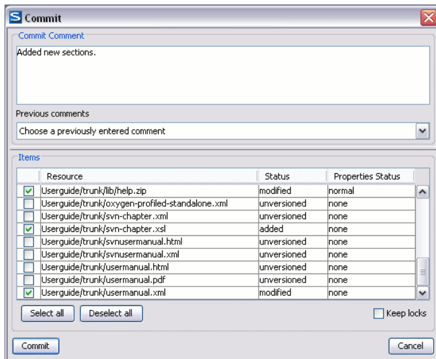
Figure 14.20. Commit dialog
