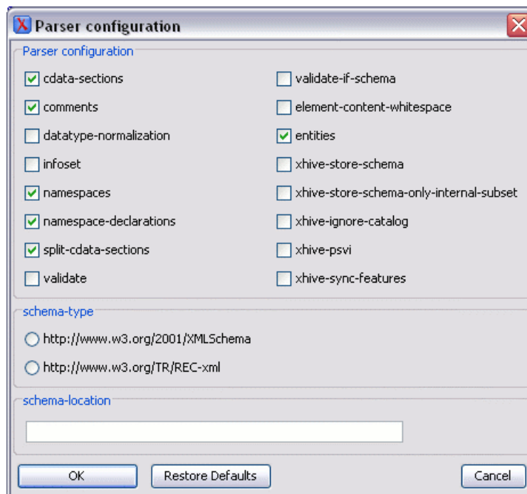
Figure 10.22. Parser configuration
