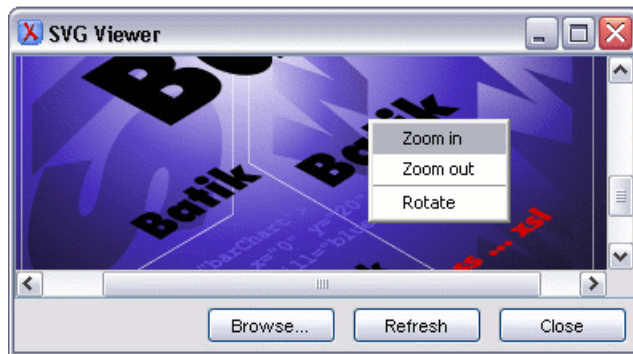
Figure 4.97. SVG Viewer
