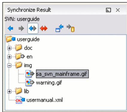
Figure 14.15. Synchronize View
