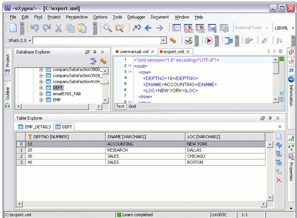
Figure 3.7. Database perspective
