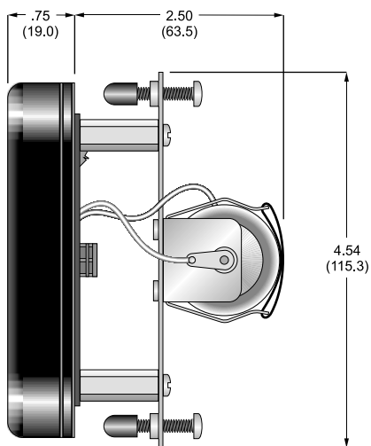
FIGURE 6 Dimensions
