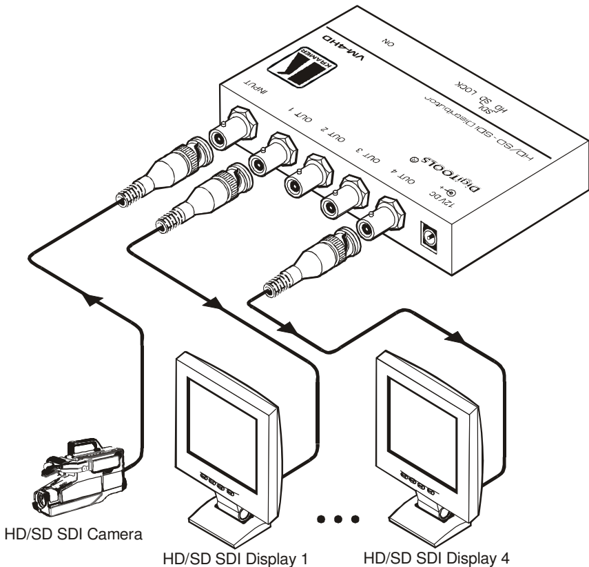
Figure 2: Connecting the VM-4HD HD/SD - SDI Distributor
