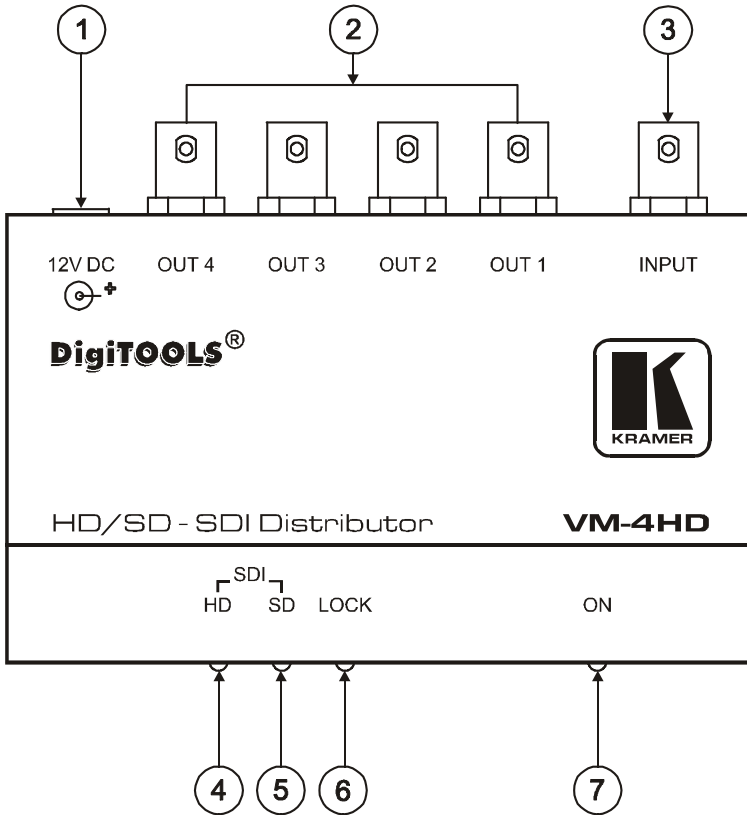
Figure 1: VM-4HD HD 1 /SD 2 - SDI Distributor
