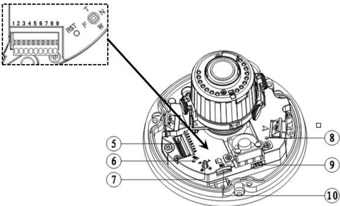
Figure 2-6 Motorized focus camera internal with IR (1-a)
