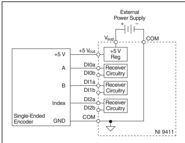
Figure 5. Connecting a Single-Ended Encoder to the NI 9411
