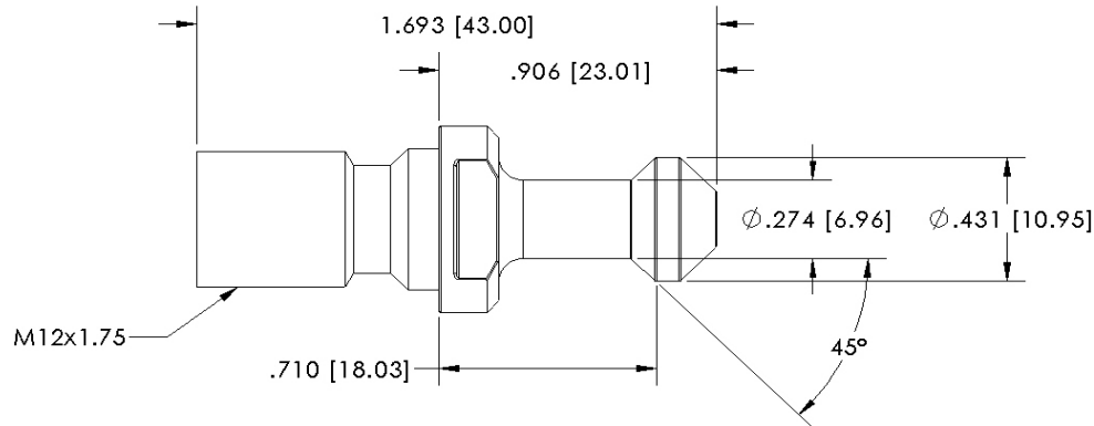
Figure 5. STC1510 Retention Knob
