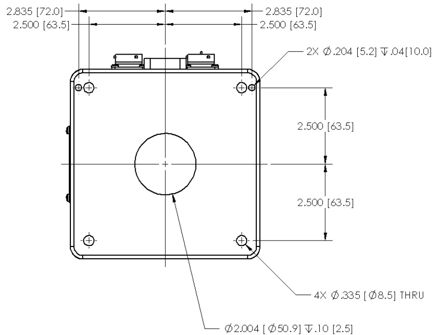
Figure 3. STC1510 Mounting Dimensions
