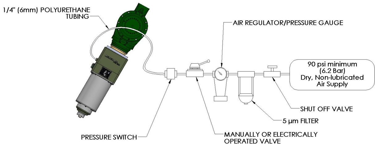
Figure 6. Pneumatic Connections
