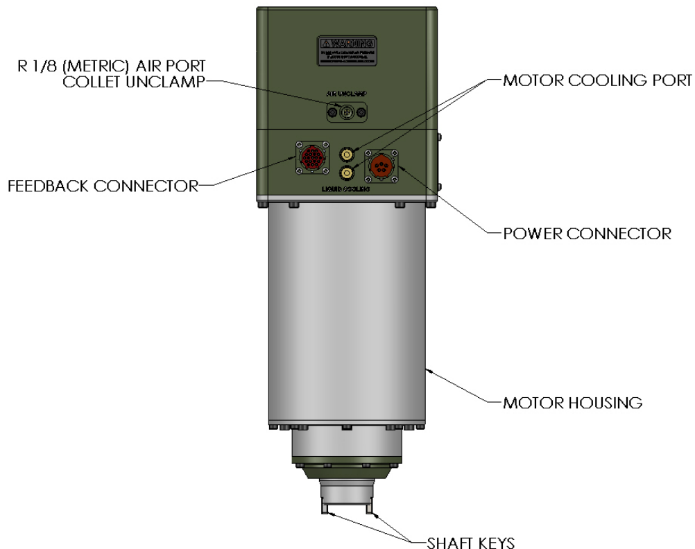
Figure 7. STC1510 External Connections
