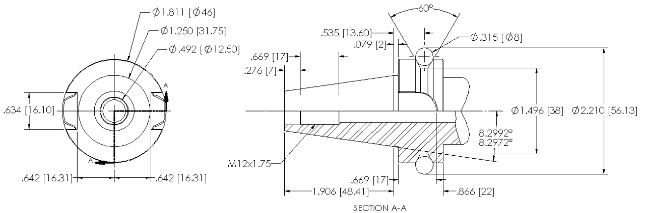
Figure 4. Toolholder Dimensions
