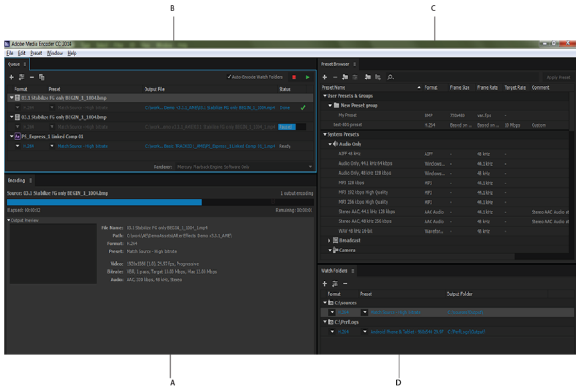
A Encoding panel B Queue panel C Preset Browser D Watch Folder
