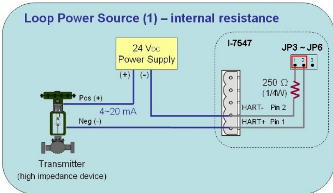
Ex1 : Loop Power Source (Internal Resistance)
