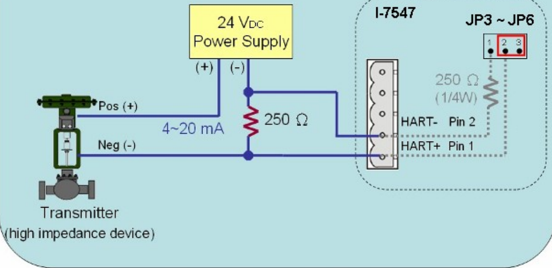
Ex2 : Loop Power Source (External Resistance)
