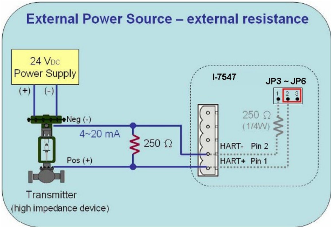
Ex4 : External Power Source (External Resistance)
