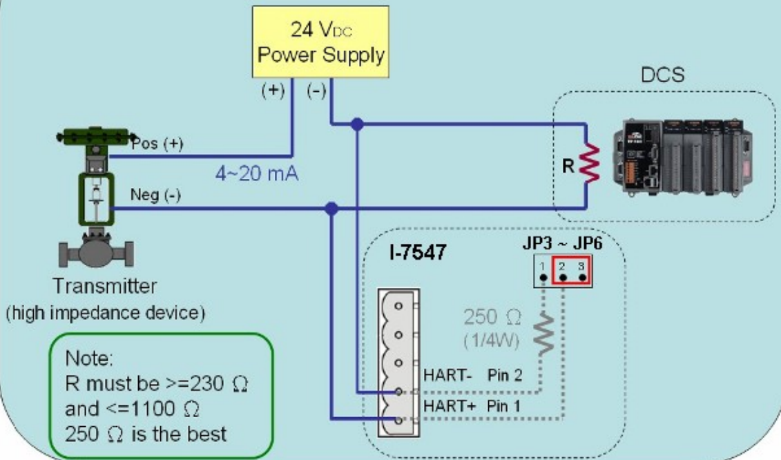
Ex3 : Loop Power Source (External Resistance)
