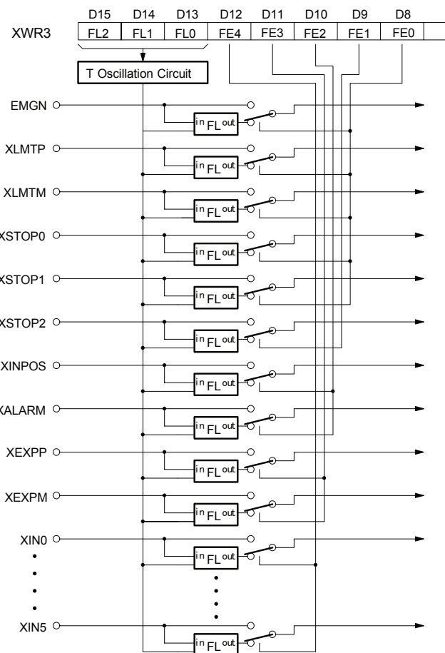
Fig. 2.29 Concept of Input Signal Filter Circuit
