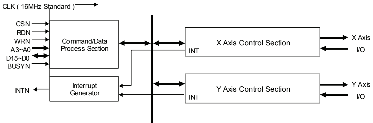
Fig. 1-1 MCX302 Functional Block Diagram
