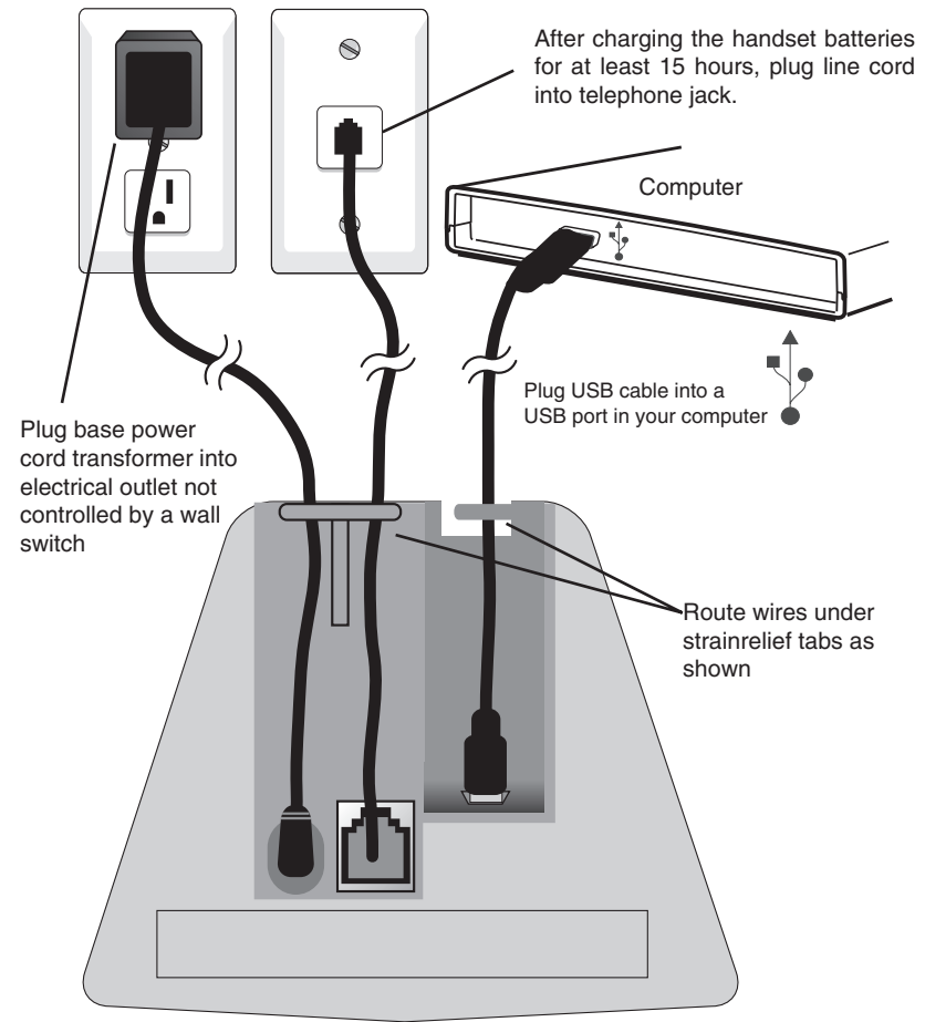
Underside of telephone base
