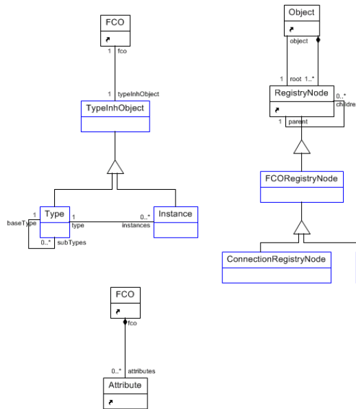
Figure 44. Relationships of Attributes, Type-Inheritance Objects and RegistryNodes
