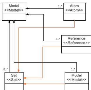
Figure 31. Example of a Set
