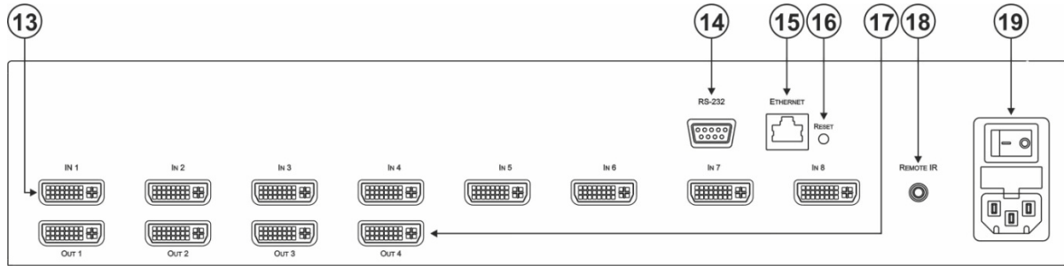
Figure 2: VS-84HDCPxI 8x4 DVI Matrix Switcher Rear Panel
