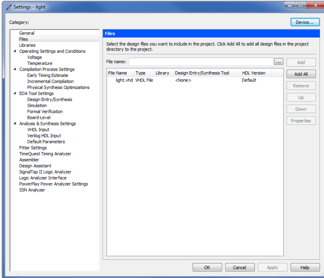
Figure 16. Settings window.
