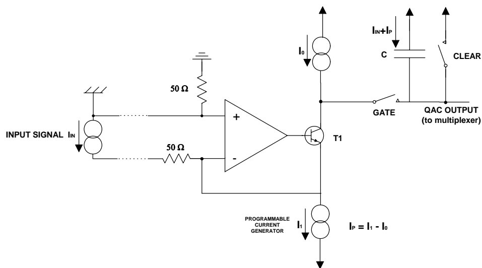
Fig. 2.3: QAC section
