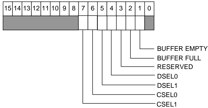
Fig. 4.23: Status Register 2
