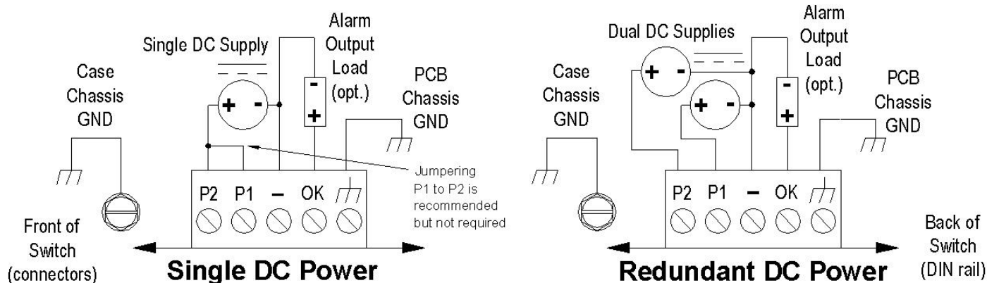
Power and Alarm Wiring for SLX-3EG-1 Managed Switches
