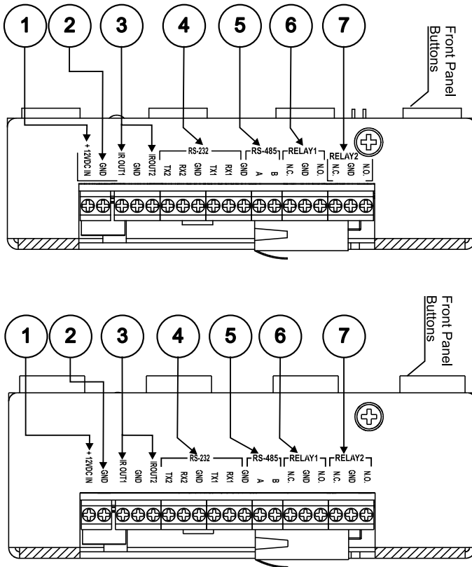
Figure 3: RC-8RK and the RC-8RKL Lower Rear Panel
