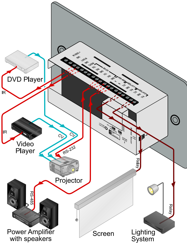
Figure 6: Example of a Typical RC-8RK / RC-8RKL Configuration
