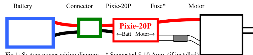
Fig 1: System power wiring diagram * Suggested 5-10 Amp (if installed)
