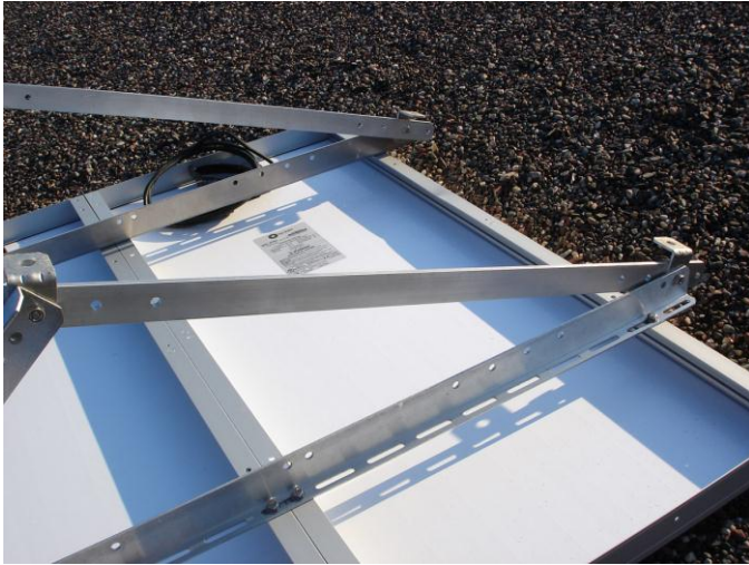
Figure 46: Assemble the Support Bar to the Mounting Frame
