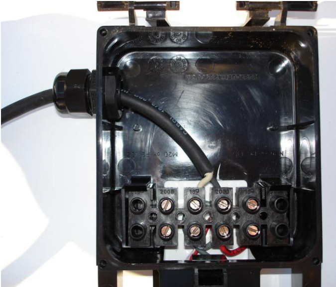
Figure 42: Secure Terminal Block and Tighten Strain Relief
