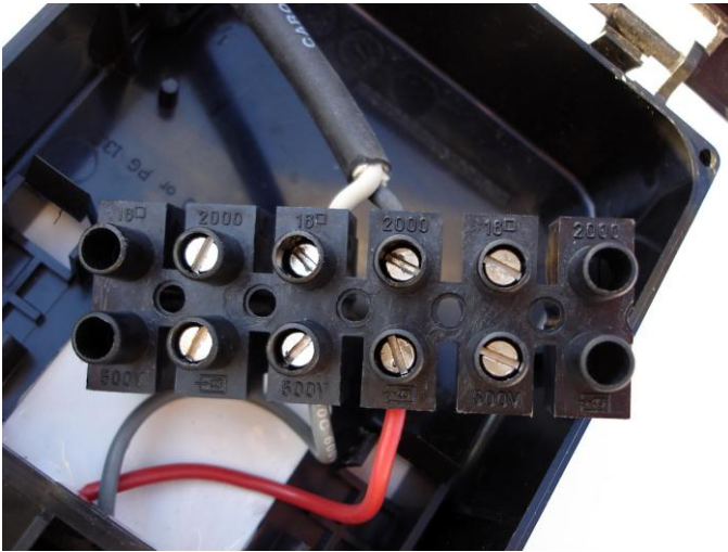
Figure 41: Power Cable Connection to Solar Cell Terminals
