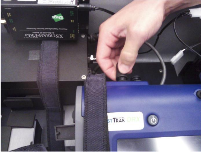
Figure 29: Connect Monitor Power Cable to DustTrak Monitor
