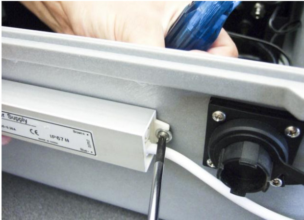
Figure 24: Attach the Adapter to the Enclosure
