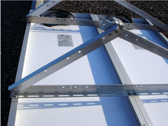
Figure 45: Assemble the Solar Cells on the Mounting Frame
