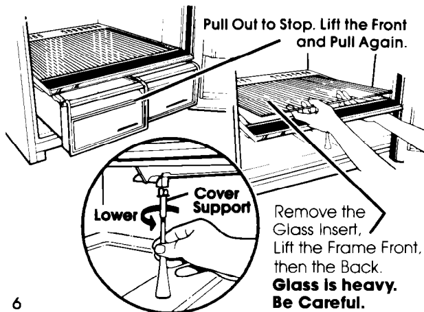
Frame Support
