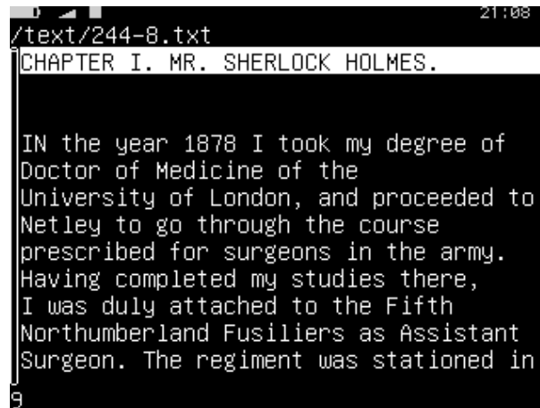
Figure 11.46.: A bookmark
