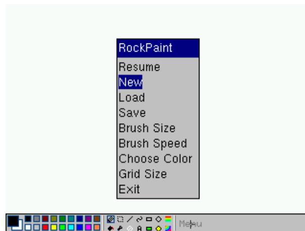
Figure 11.53.: Rockpaint
