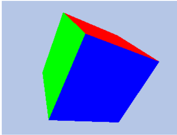
Figure 11.32.: Cube
