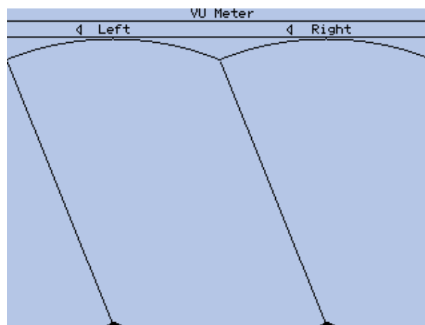
Figure 11.42.: VU-Meter
