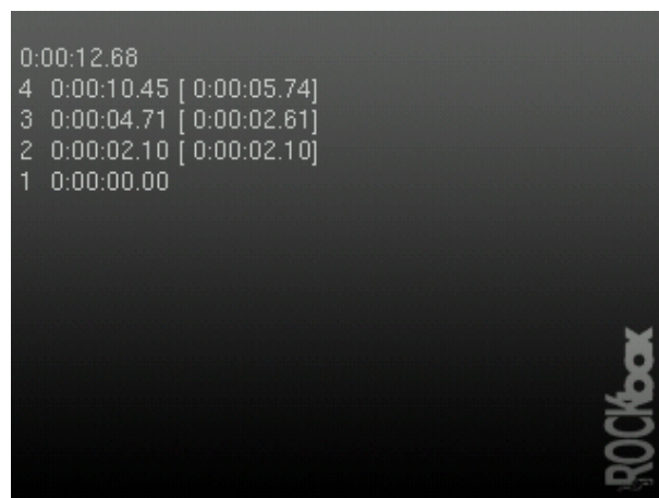
Figure 11.55.: Stopwatch
