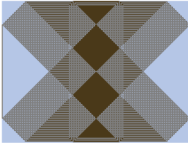
Figure 11.36.: Mosaïque
