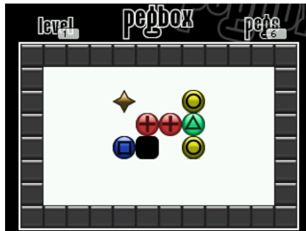
Figure 11.17.: pegbox
