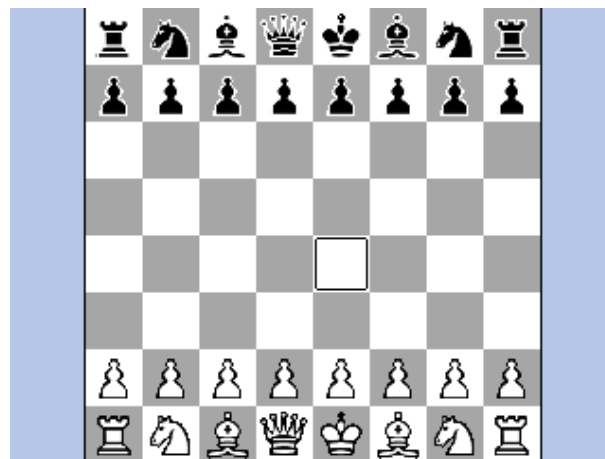
Figure 11.4.: Chessbox
