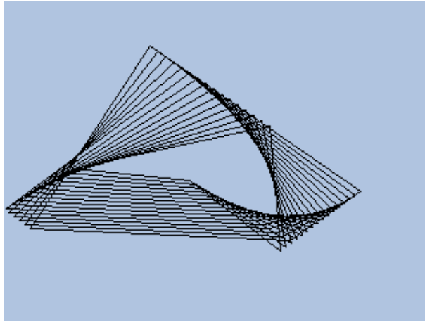
Figure 11.33.: Demystify
