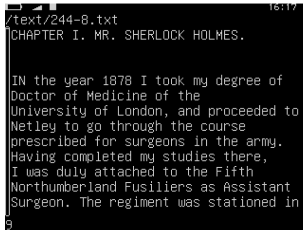
Figure 11.44.: Text Viewer
