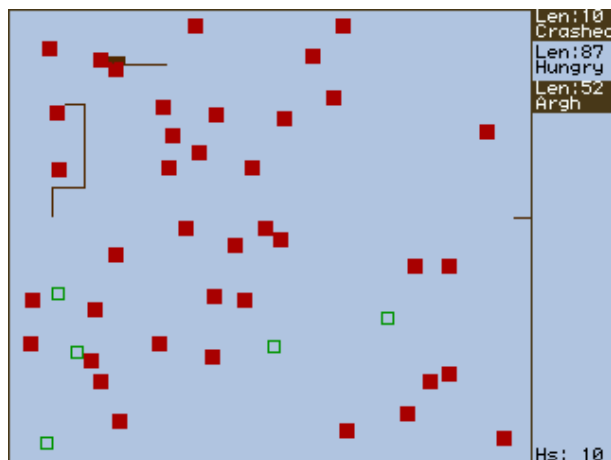
Figure 11.29.: Wormlet game
