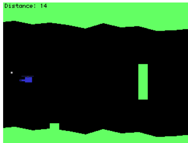
Figure 11.6.: Chopper
