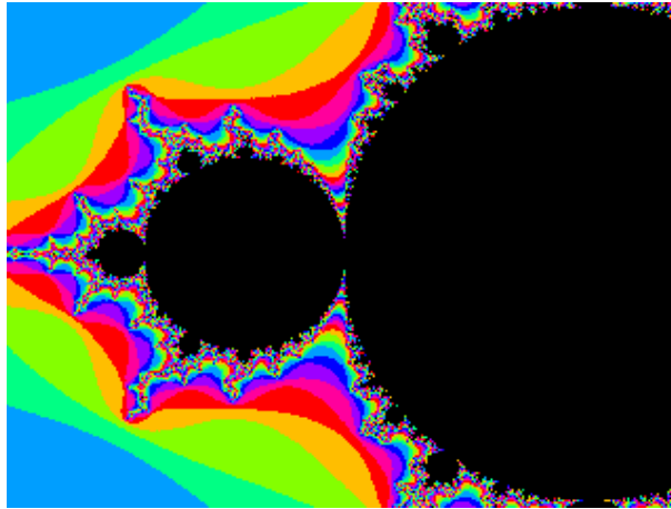
Figure 11.35.: Mandelbrot
