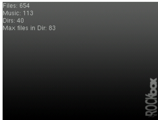
Figure 11.54.: The stats-plugin
