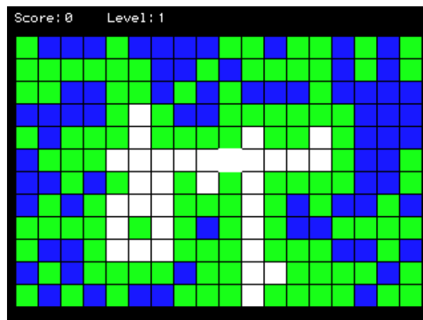
Figure 11.5.: Clix
