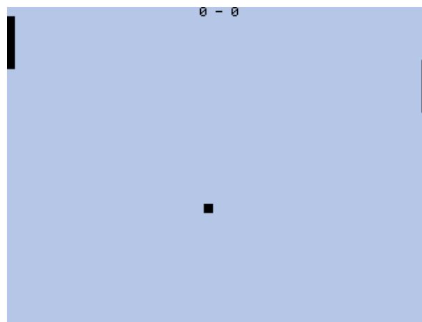
Figure 11.18.: Pong
