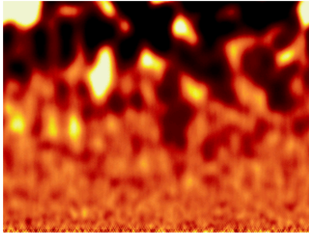
Figure 11.34.: Fire
