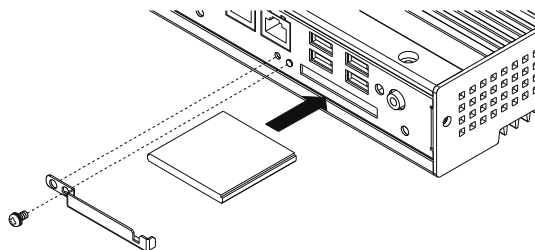
Figure 3.1. Attaching the CFast Attachment Fittings
