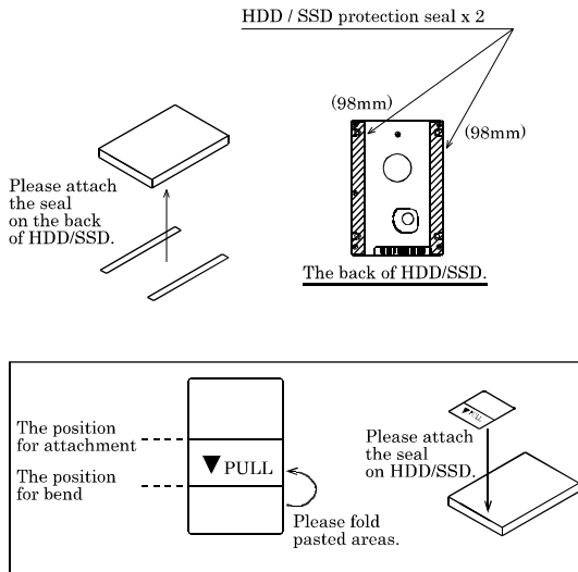
Figure 3.7. Pasting HDD/SSD protection seal and HDD/SSD removal seal
