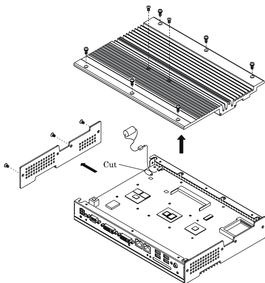
Figure 6.1. Removing the battery
