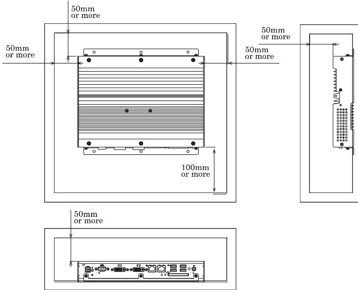
Figure 3.11. Distances between this product and its vicinity
