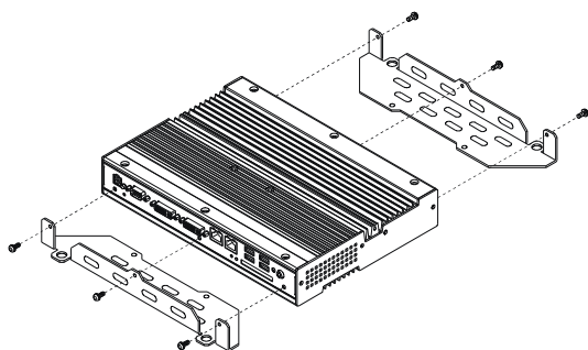
Figure 3.9. Installation of VESA metal fittings
