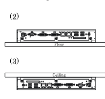
Figure 3.10. Installation Orientation (BX-961D)
