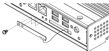
Figure 3.2. Attaching the CFast Cover
