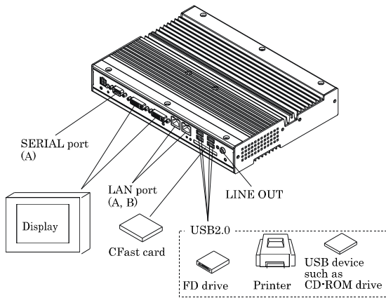
Figure 4.2. System Configuration
