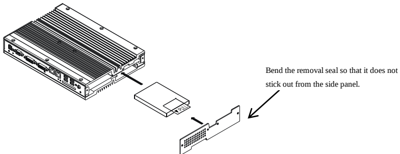
Figure 3.8. Installation of HDD/SSD
