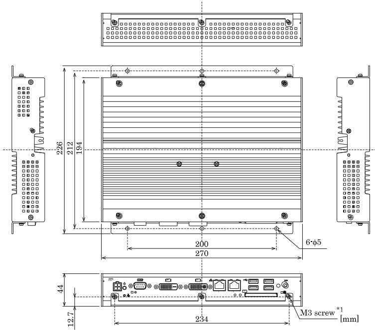
Figure 2.1. Physical Dimensions < BX-961D >
