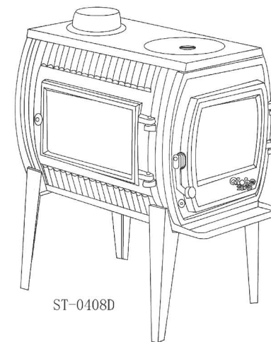
Charon II
