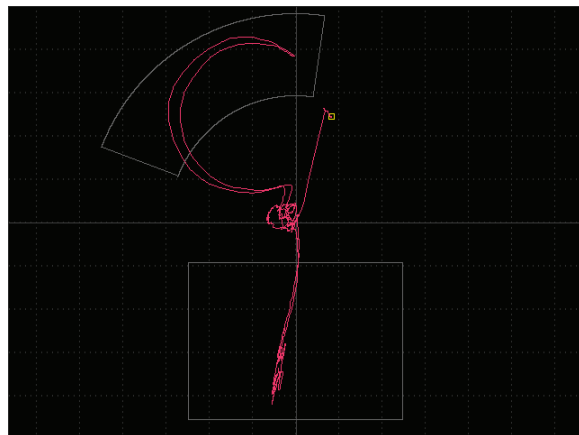
MIA mode configured to identify repaired area (bottom signal) as opposed to disbanded condition (top signal).
