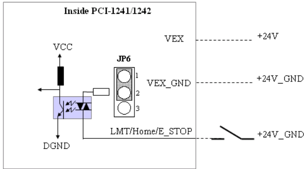
Figure 3.9: Local Input Wiring Diagram
