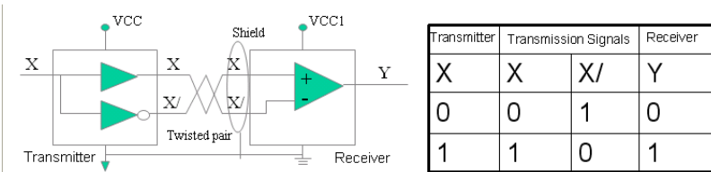
Figure 3.6: Differential Signal Transmission Method
