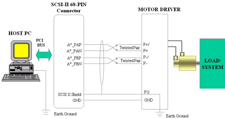
Figure 3.5: Wiring Diagram between PCI-1241 and Servo Motor Driver
