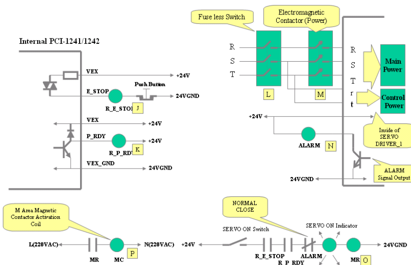
Figure 3.12: Local I/O Wiring Example of Axis One (II)
