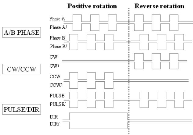
Figure 3.7: Pulse Output Format
