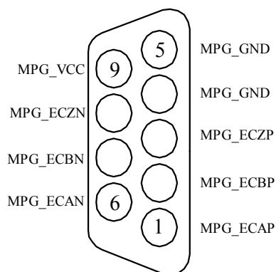
Figure 3.13: MPG Encoder Input DB-9 Connector Pin Assignment
