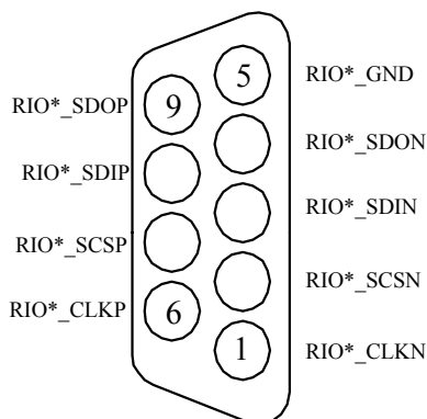
Figure 3.15: Remote I/O DB-9 Connector Pin Assignment
