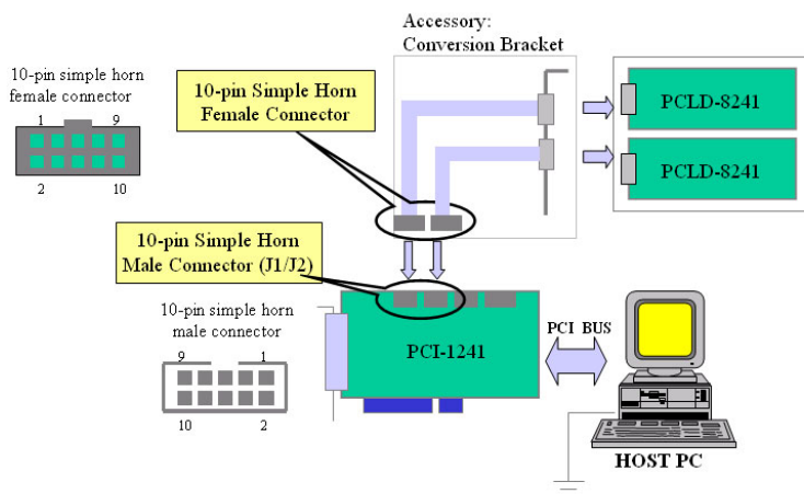
Figure 3.16: Remote I/O Wiring Diagram in PCI-1241
