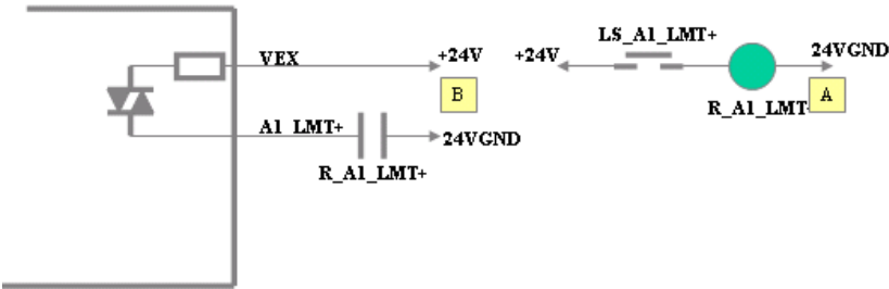
Internal PCI-1241/1242
