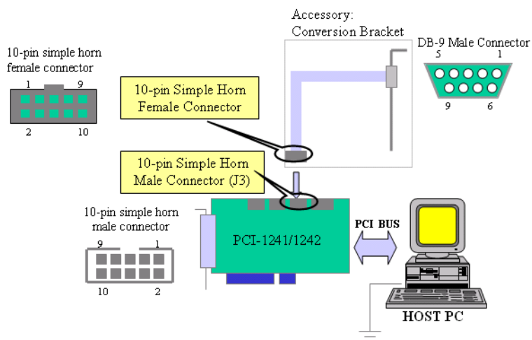
Figure 3.14: MPG Encoder Input Wiring Diagram
