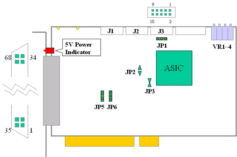
Figure 2.2: Location of Jumpers and VRs on PCI-1241/42
