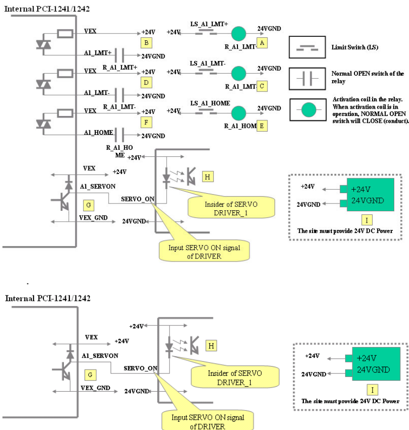
Figure 3.11: Local I/O Wiring Example of Axis One (I)
