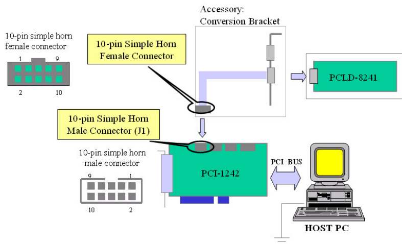
Figure 3.17: Remote I/O Wiring Diagram in PCI-1242
