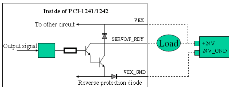
Figure 3.10: Local Output Wiring Diagram
