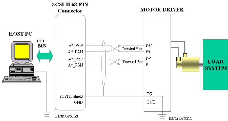
Figure 3.8: Wiring Diagram Between PCI-1241/42 and Pulse-Type Driver
