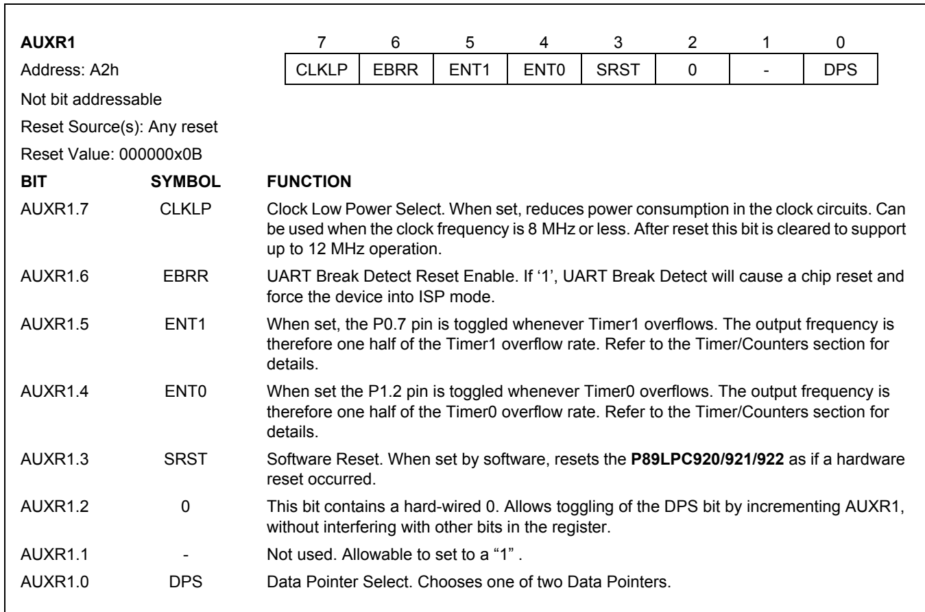
Figure 14-1: AUXR1 register
