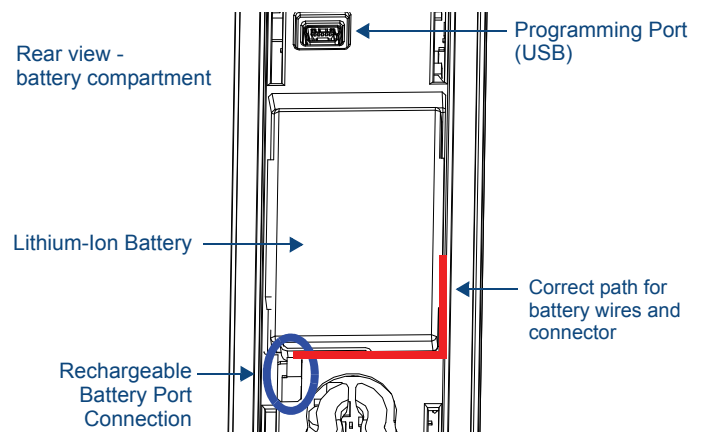
FIG. 2 Rechargeable Battery and Programming Ports on The Mio R-4 Remote
