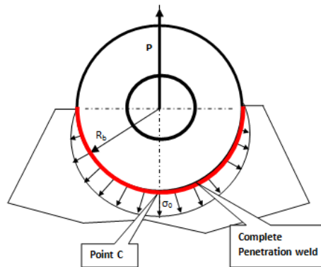
Figure J.12 – Vertical loaded boss
