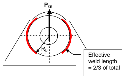
Figure J.10 – Effective weld length
