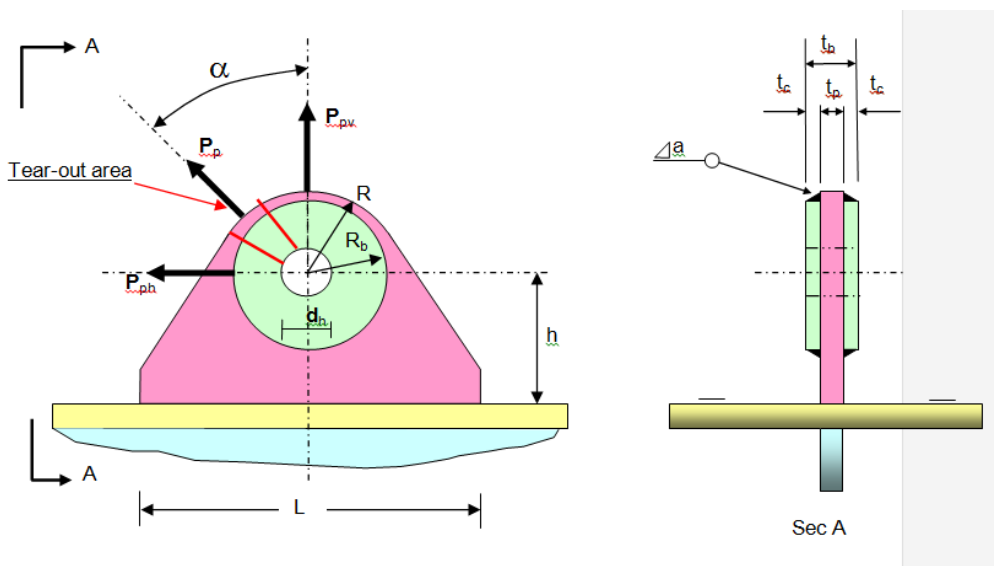
Figure J.8 - Design load components
