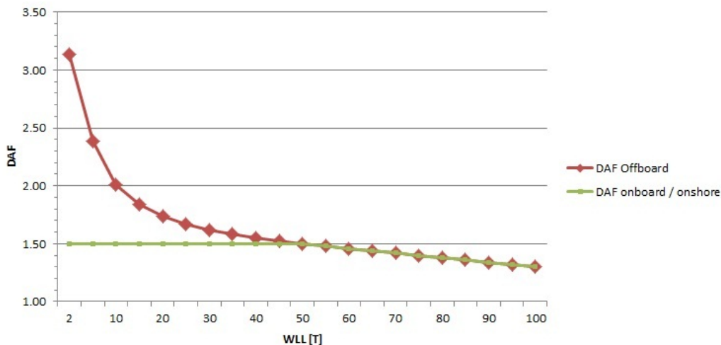
Figure F.4 – Dynamic amplification factor (DAF)
