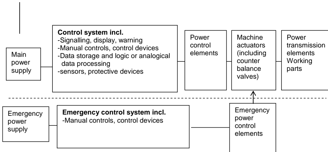
Figure G.1 Schematic representation of EOS
