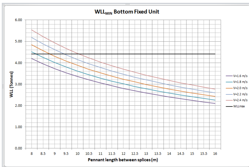
Figure I.4 WLL variation for a specific rope to be used on a bottom fixed unit
