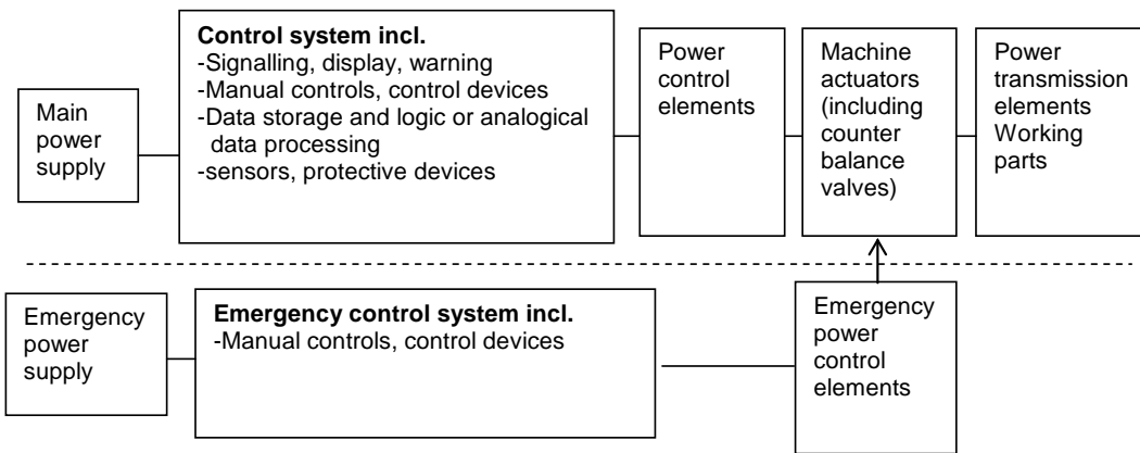
Fig. 1 Independency of emergency operation system- NOTE For terminology, see EN ISO 12100.
