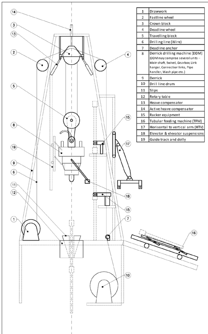
Figure D.1 – Conventional drawwork including top drive/DDM
