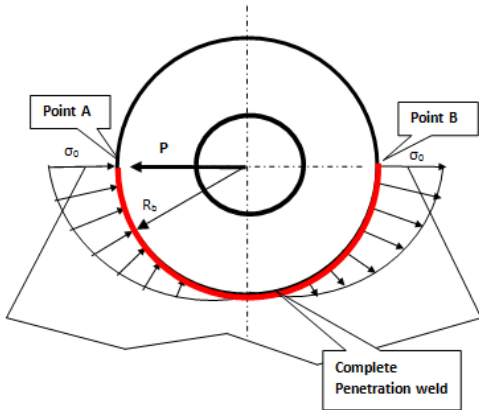
Figure J.11 – Horizontal loaded boss
