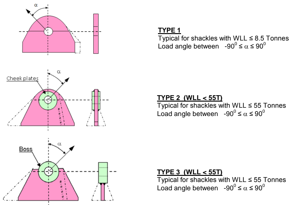
Figure J.1 - Lifting lugs Type 1, 2 and 3 (Dotted lines indicate alternative designs)
