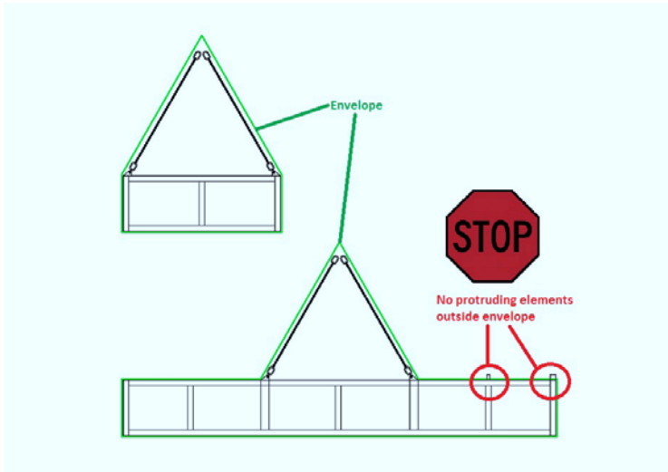
Figure F.1 - Envelope of unit represented by frame and sling arrangement
