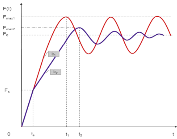
Figure A.1 - Effect of shock absorber
