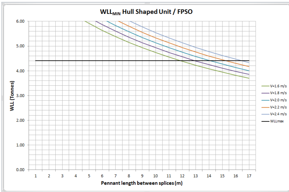
Figure I.6 WLL variation for a specific rope to be used on a monohull shaped unit / FPSO
