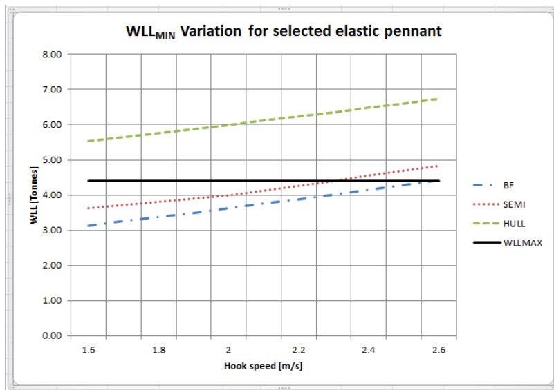
Figure I.3 WLL variation
