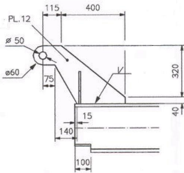
Figure H.1—Typical installation: Example of arrangement for installation of hoists and trolley with self weight up to 500 kg. Special consideration of installation Installation arrangement capacity shall be given to power driven hoists for trolley and beam hoist is to be marked with large SWL and tested accordingly, ref. H.6.
