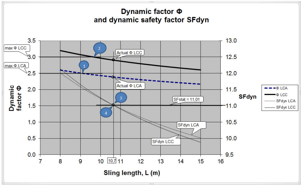
Figure I.2 – Dynamic factor, \Phi , and dynamic safety factor, SF_{dyn} , plotted against sling length
