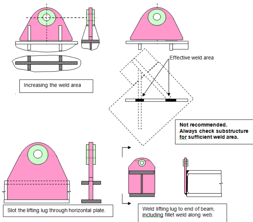
Figure J.3 - Welded connections
