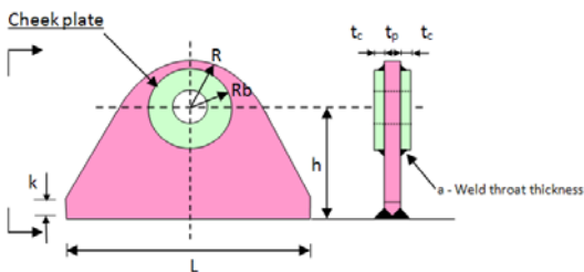
Figure J.6 - Lifting lug Type 2 geometry – Cheek plates each side
