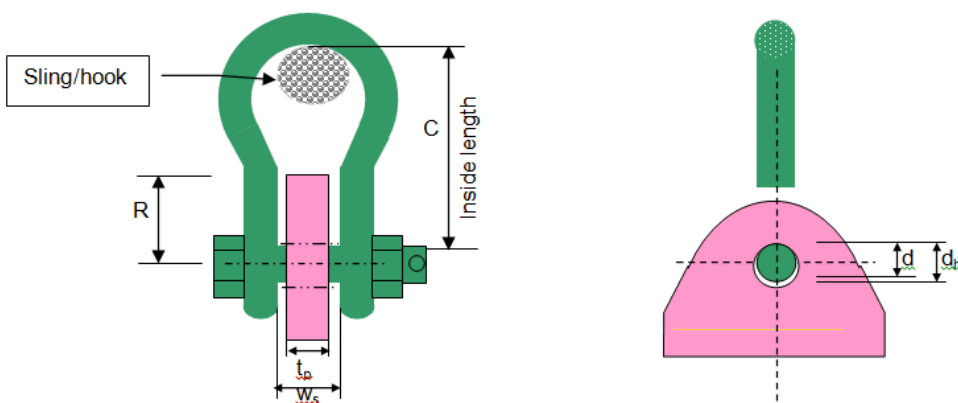
Figure J.4 - Lifting lug vs. shackle interface - Type 1 Lifting lug shown
