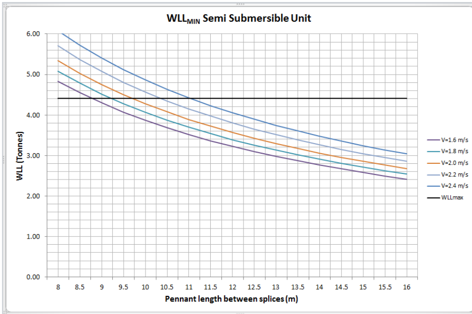
Figure I.5 WLL variation for a specific rope to be used on a semisubmersible unit
