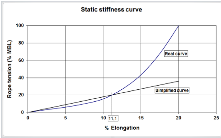
Figure I.1 – Rope static stiffness curve
