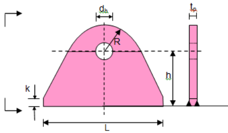
Type 1 – Load Angle - 90^0 \leq \alpha \leq 90^0
