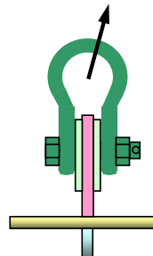
Figure J.9 Lateral load acting in the centre of the shackle bow
