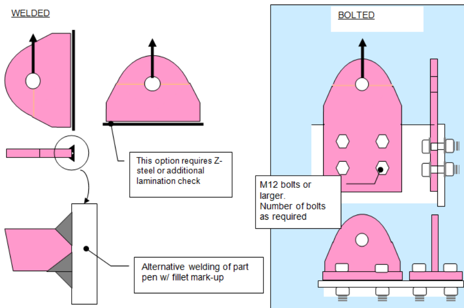
Figure J.2 - Welded/bolted connections
