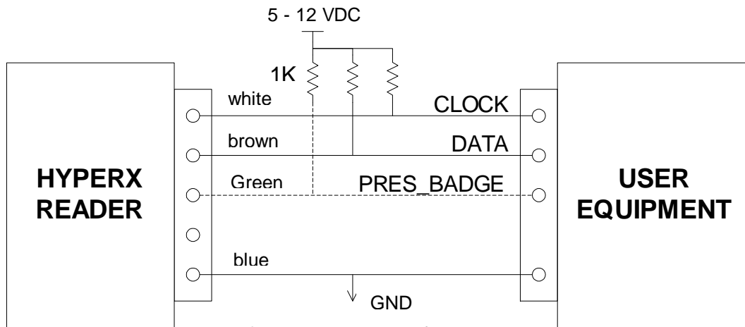
ISO2 (DATA/CLOCK) reader connection
