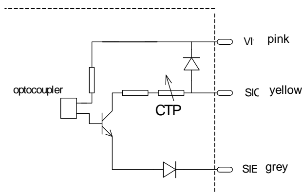
Circuit diagram of the digital output
