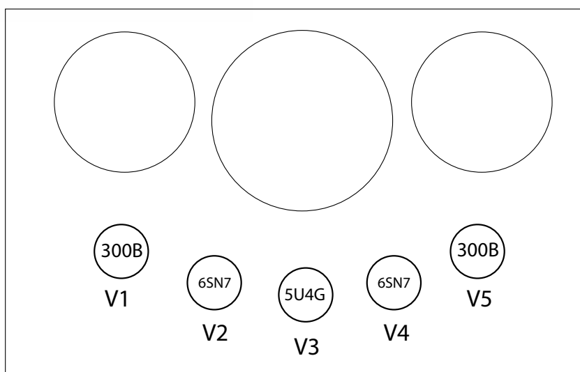
Figure 1: Experience Two tube layout
