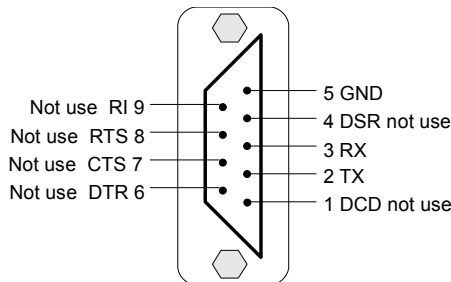
Fig. 4. RS232 interface signals of DB-9F (female) connector
