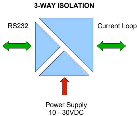
Fig. 3. Isolation structure
