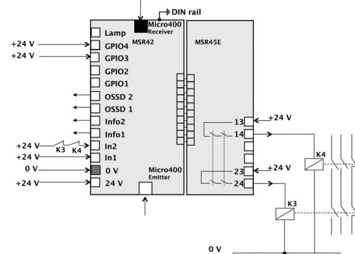
Figure 7: MSR42 base module and MSR45E expander module (basic configuration, automatic start, with start release). For teach-in see page 8
