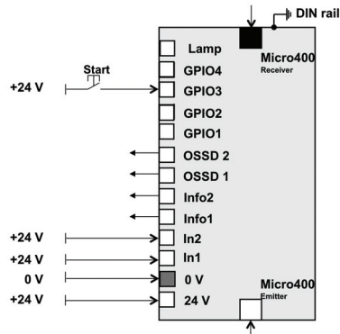
Figure 3: MSR42 base module (basic configuration, manual start). For teach-in see page 8
