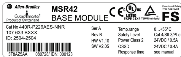
Figure 14: Product label MSR42 control module
