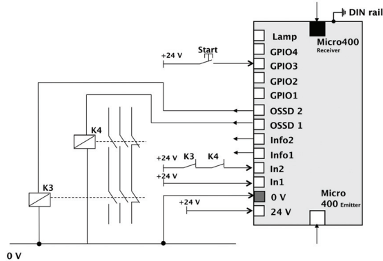
Figure 4: MSR42 base module (basic configuration, manual start, with start release). For teach-in see page 8
