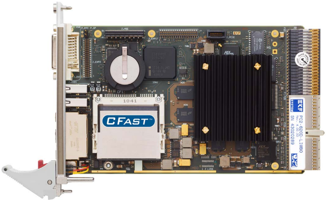
PC2-LIMBO (Top View)
