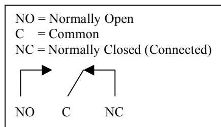
Fig. 3: Relay contacts (in the inactive state)
