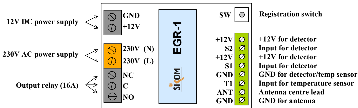
Fig. 1: Connection terminals of EGR-1
