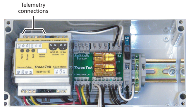
Figure 6. Telemetry Connections
