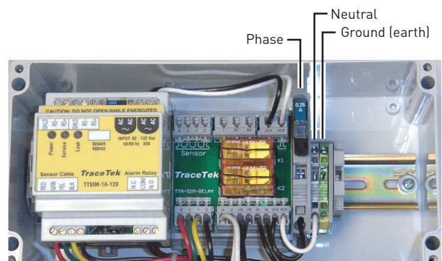
Figure 3. Power connections
