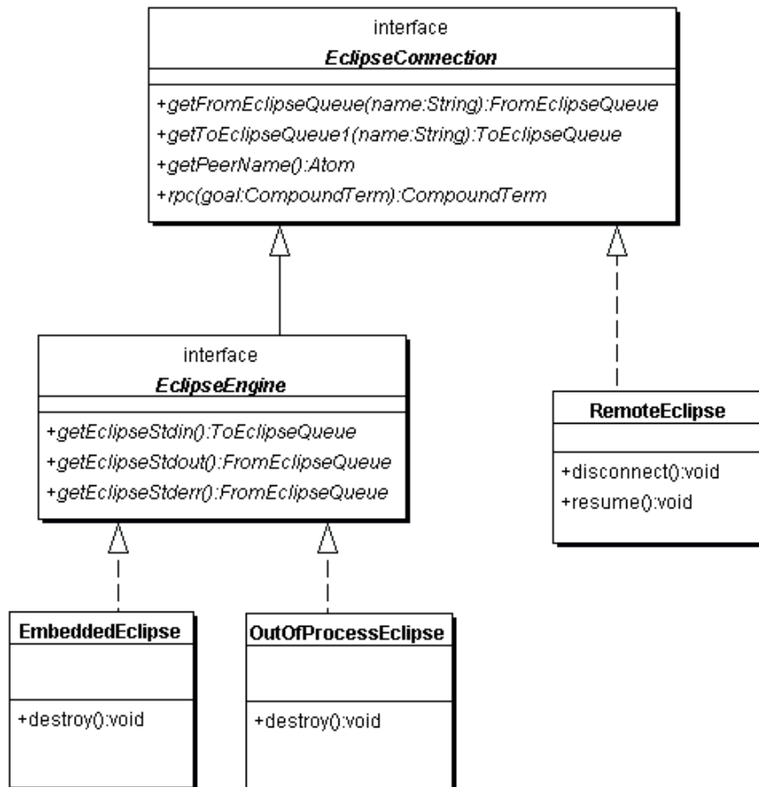
Figure 7.4: UML class diagram for different classes connecting Java and ECL i PS e . Some convenience methods from EclipseConnection have been omitted.
