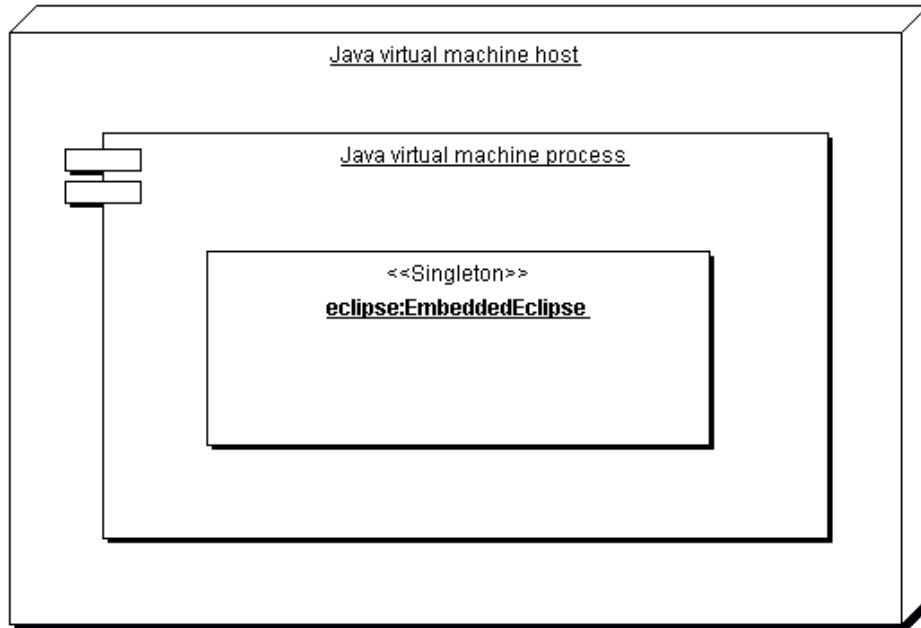
Figure 7.1: UML deployment diagram for EmbeddedEclipse
