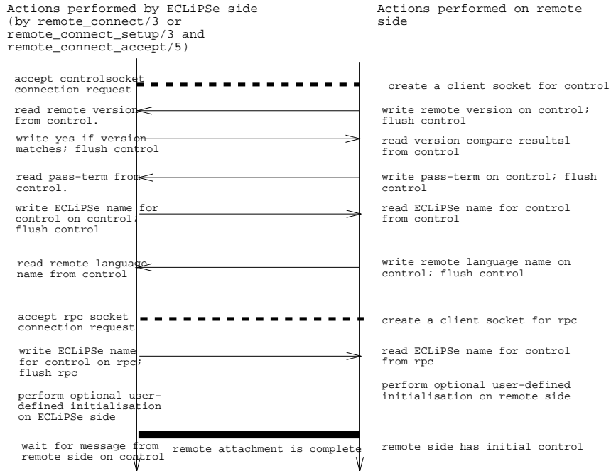
Figure 9.1: Summary of the attachment protocol
