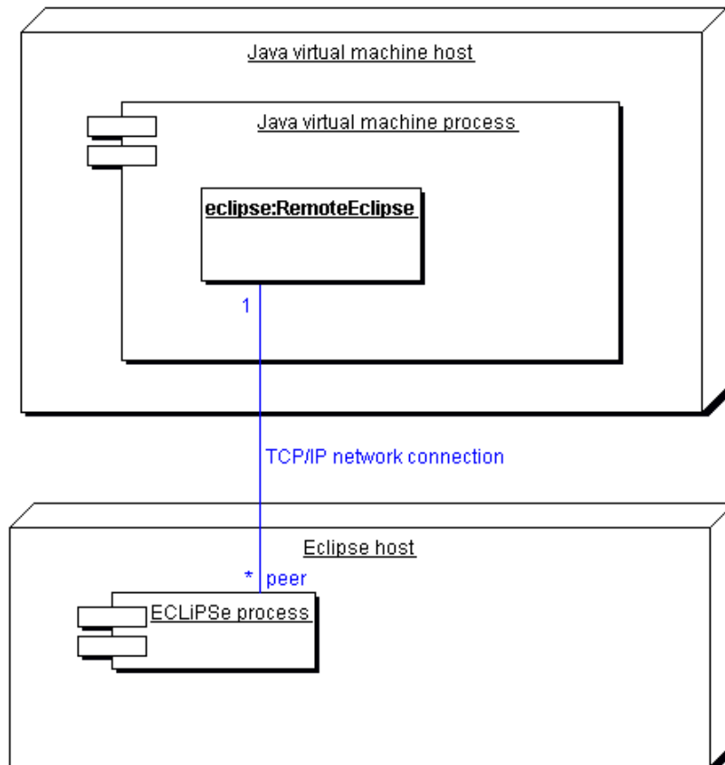
Figure 7.3: UML deployment diagram for RemoteEclipse
