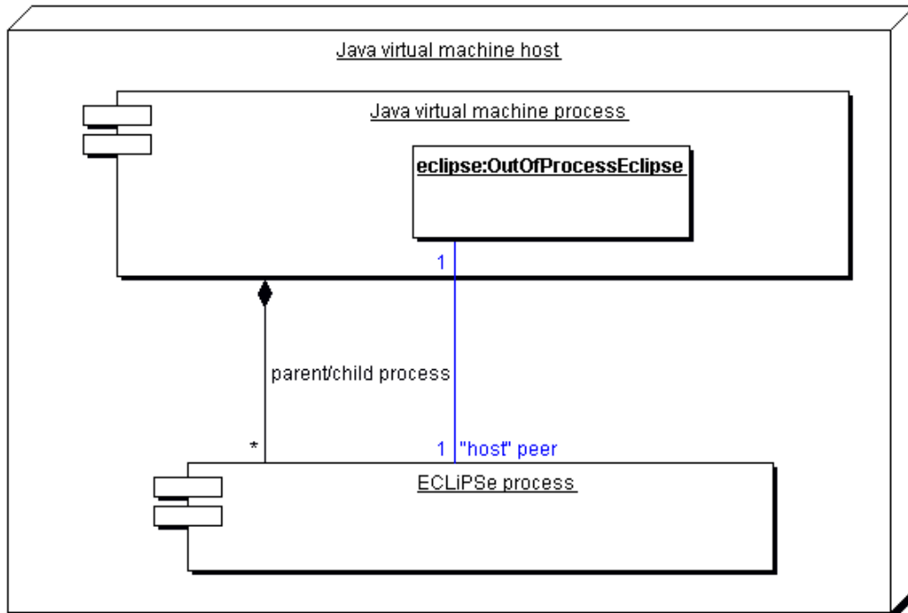
Figure 7.2: UML deployment diagram for OutOfProcessEclipse
