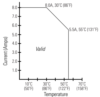
FET Total Current (1762-L40BXB and L40BXR)
